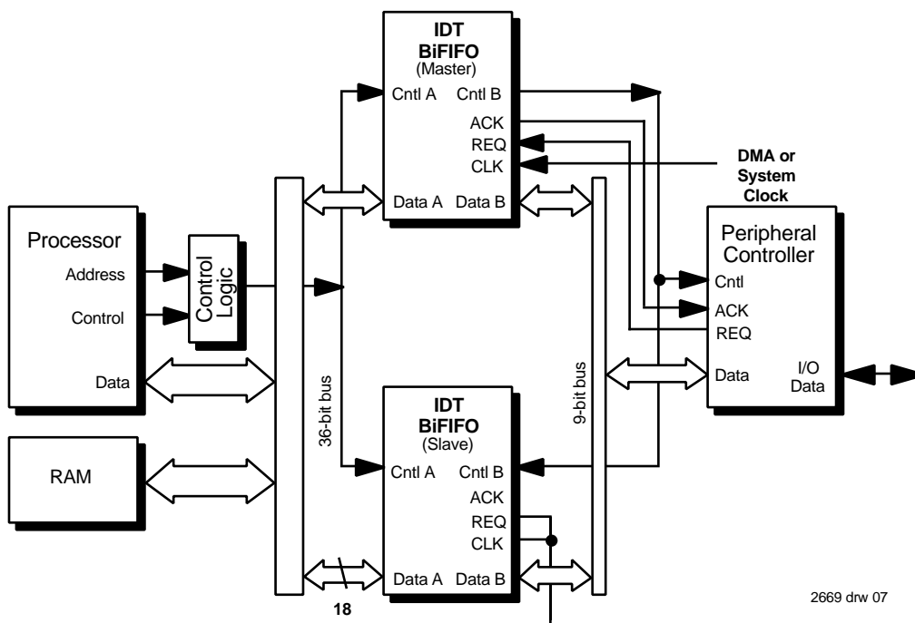
Figure 4. 36- to 9-Bit Peripheral Interface Configuration
