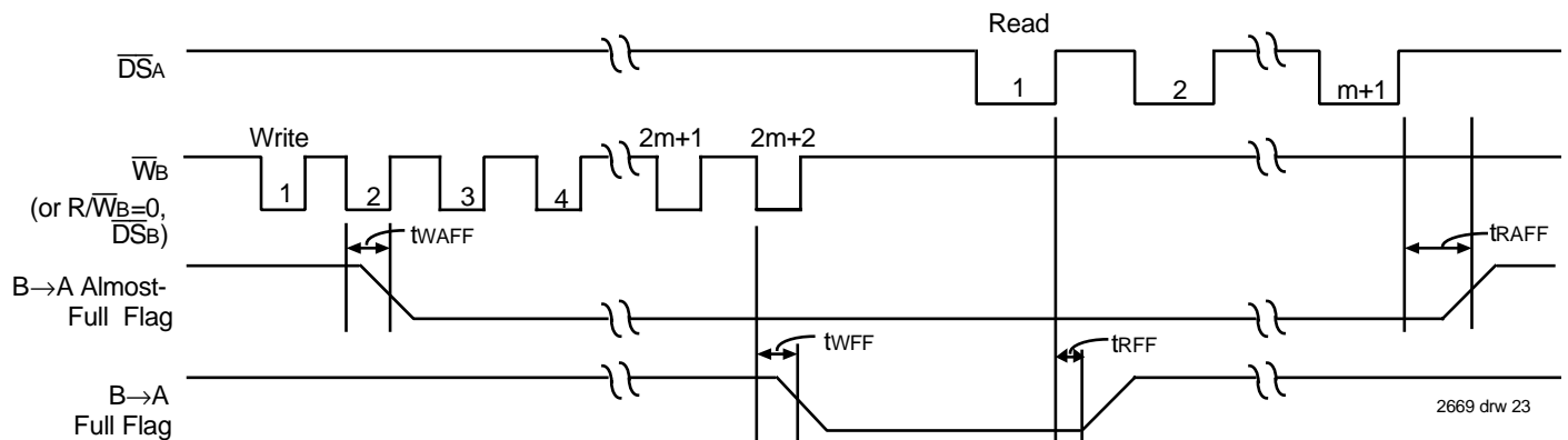
Figure 20. Empty and Almost-Empty Flag Timing for B→A FIFO. ( n = Programmed Offset)
