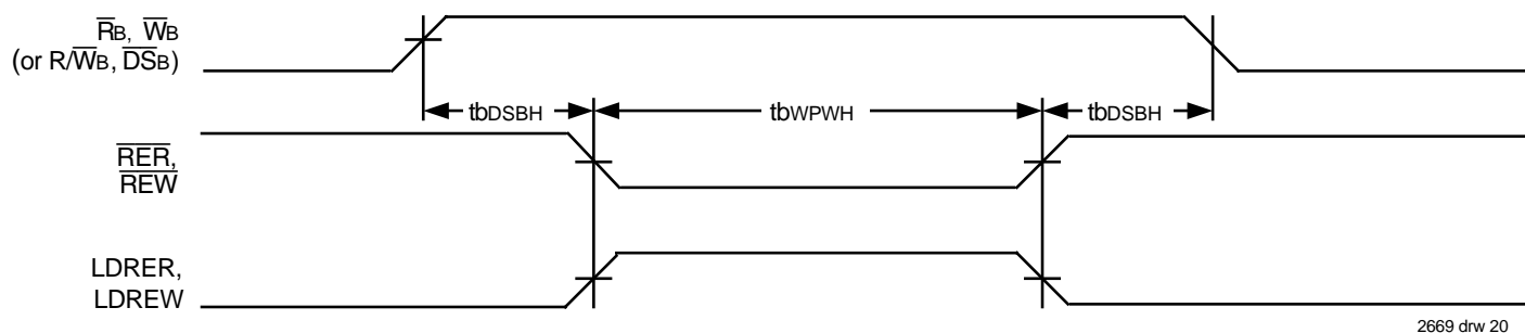
Figure 18. Port B Reread and Rewrite Timing for Intelligent Retransmit
