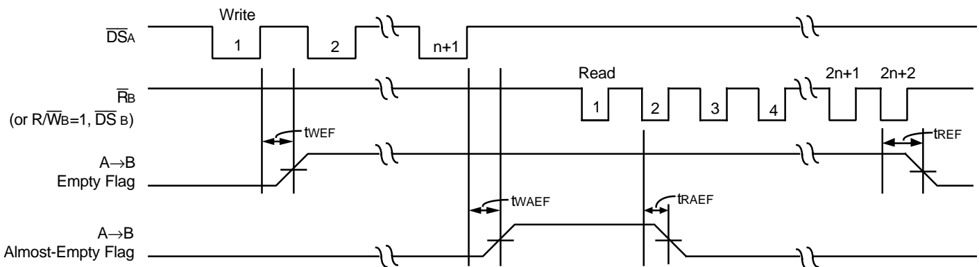
Figure 21. Full and Almost-Full Flag Timing for B→A FIFO. ( m = Programmed Offset)
