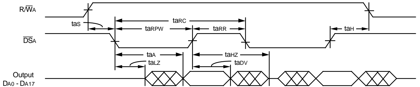
Figure 12. Read and Write Timing for Port A
