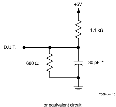
Figure 8. Output Load
