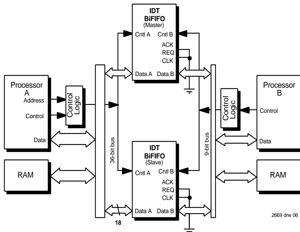
Figure 3. 36- to 9-Bit Processor Interface Configuration
