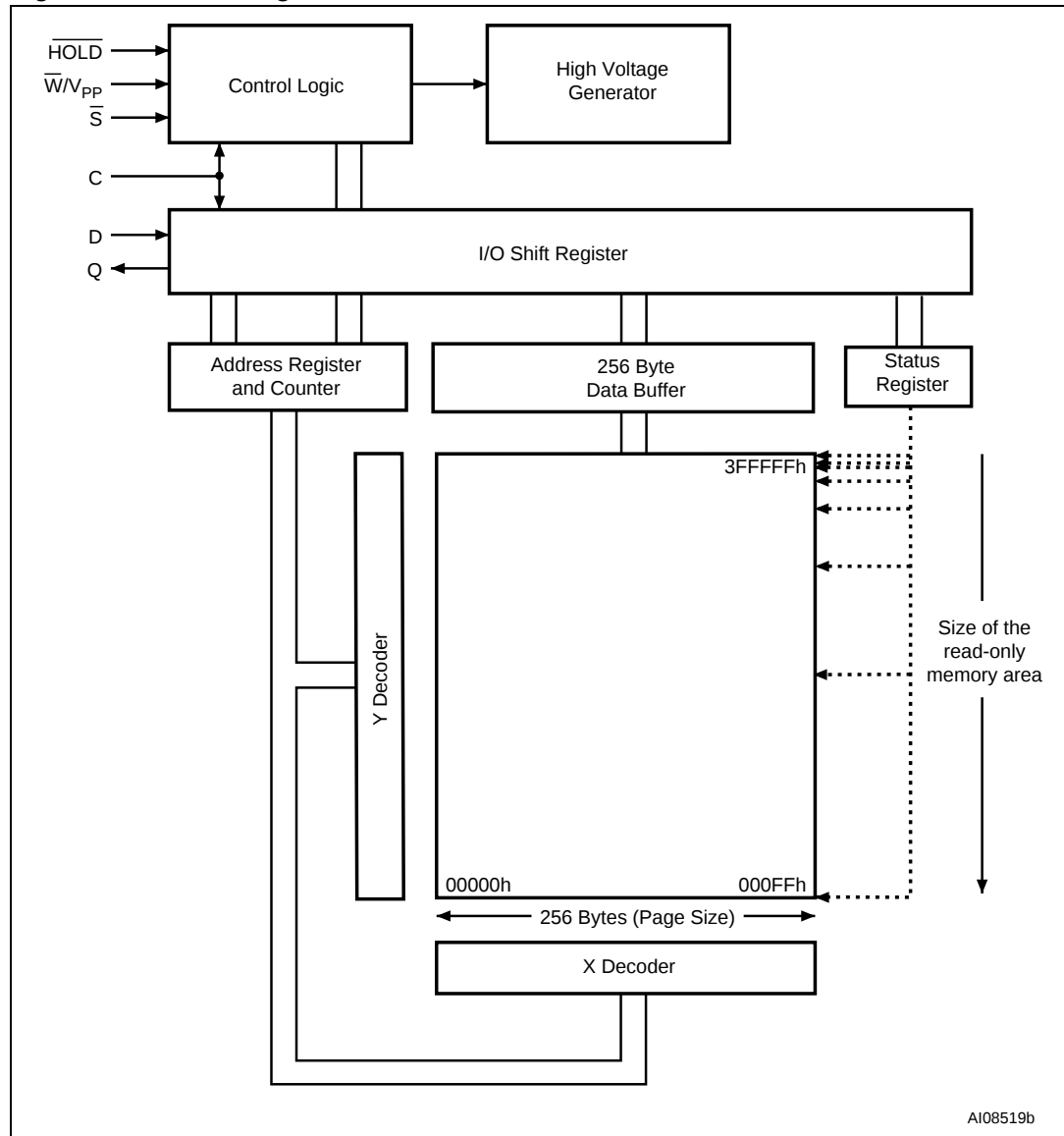
Figure 7. Block diagram
