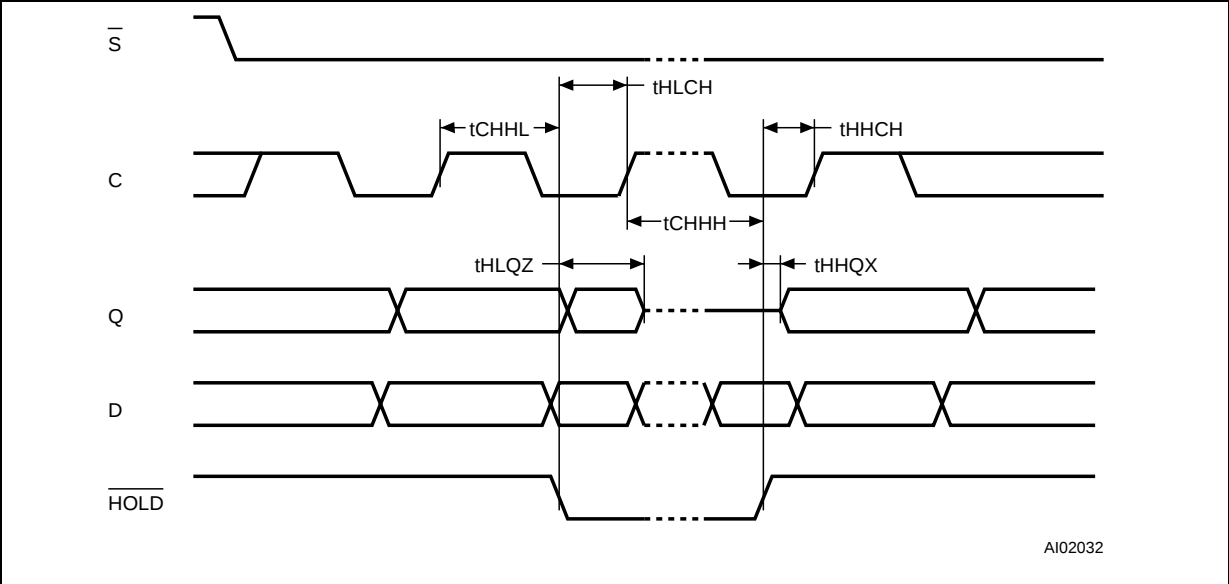
Figure 25. Hold timing
