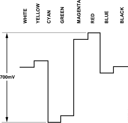
Figure 134. Pr Levels—PAL
