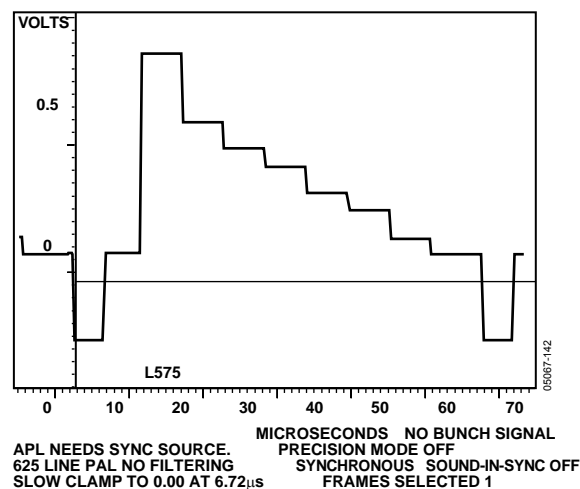
Figure 142. PAL Luma
