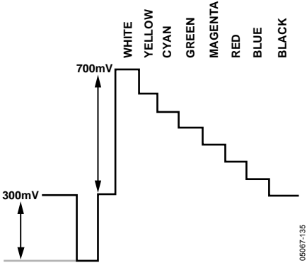
Figure 134. Pr Levels—PAL
