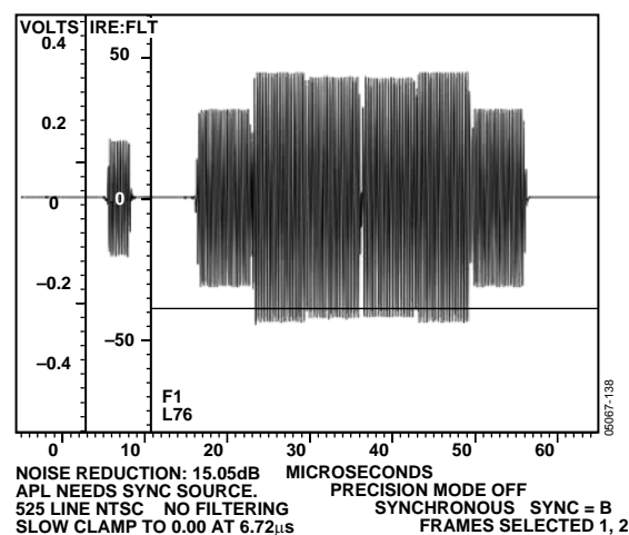
Figure 138. NTSC Chroma
