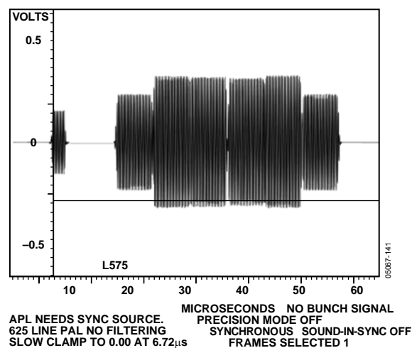
Figure 141. PAL Chroma
