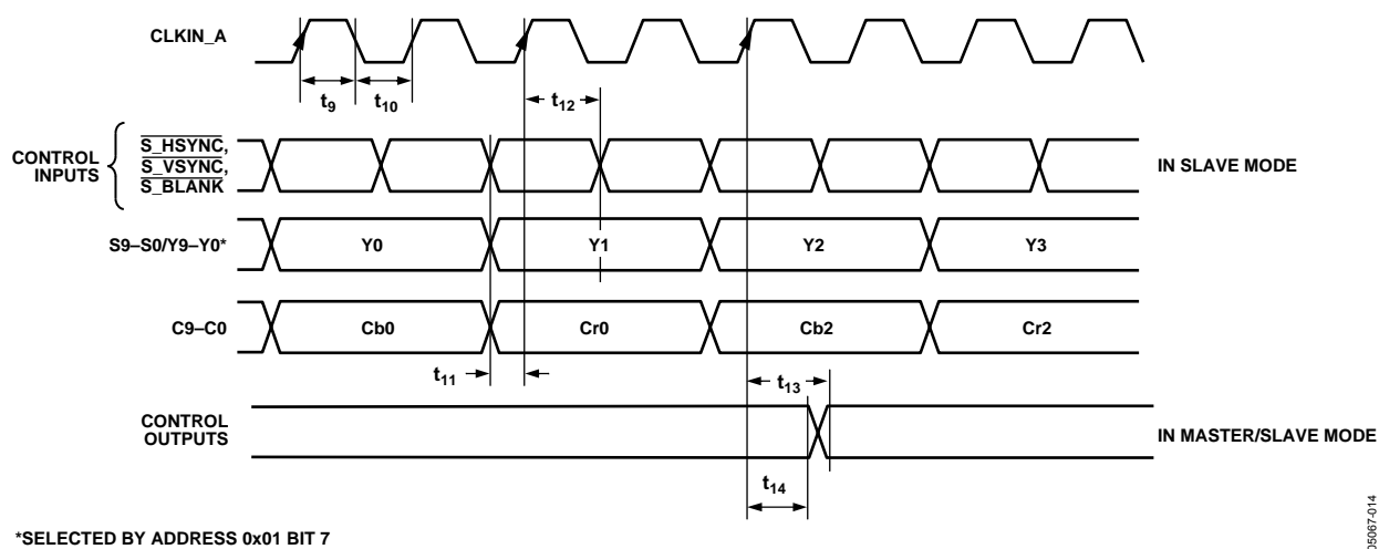
Figure 14. 20-/16-Bit SD Only Pixel Input Mode (Input Mode 000)
