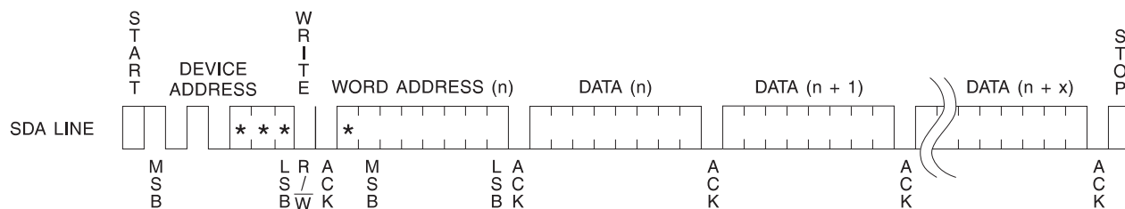
Figure 6. Page Write
