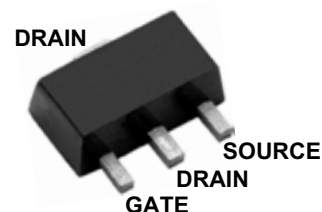
TO-243AA (SOT-89)
