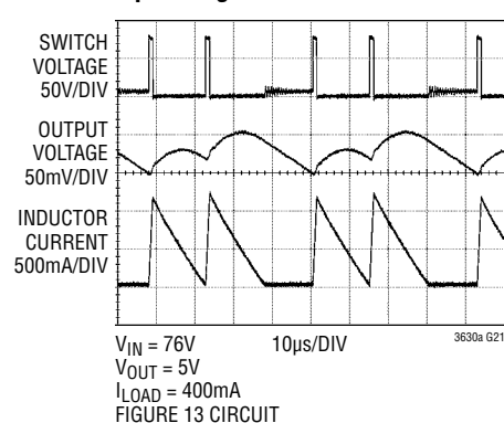
Operating Waveforms
