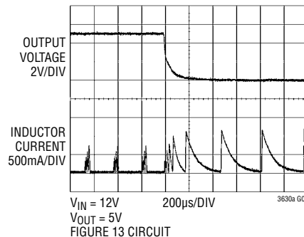
Short-Circuit Response
