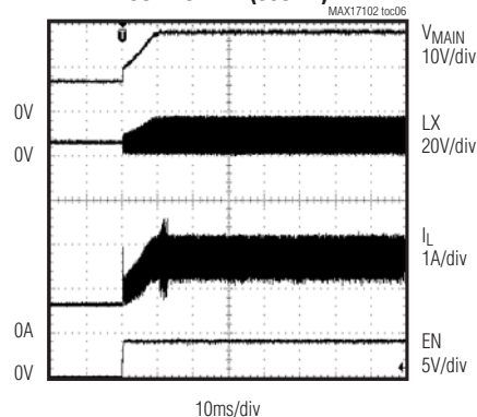
STEP-UP REGULATOR HEAVY-LOAD SOFT-START (350mA)
