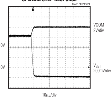
CALIBRATOR FULL-SCALE UPWARD STEP RESPONSE
