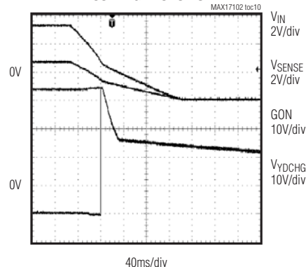
DISCHARGE FUNCTION
