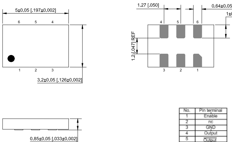
External Dimensions
