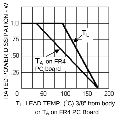
FIGURE 1 Power Derating Curve
