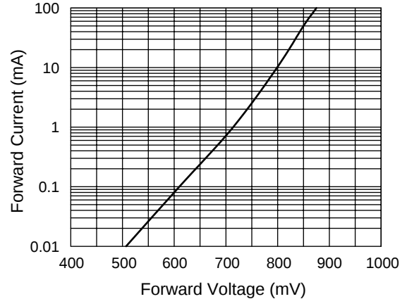
DC Characteristic
