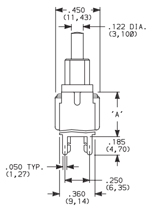
SNAP-IN
