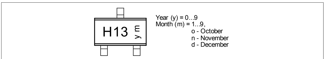
Figure 4-5 Marking of TLE4961-3K
