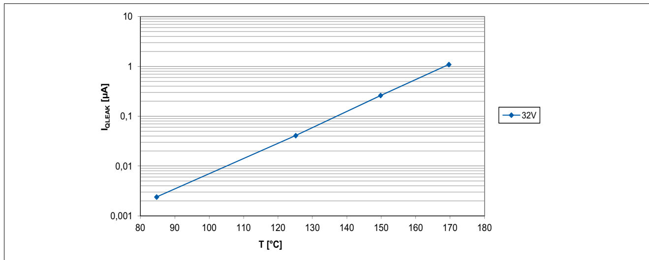
Figure 6-11 Output Leakage Current of the TLE4961-3K over Temperature
