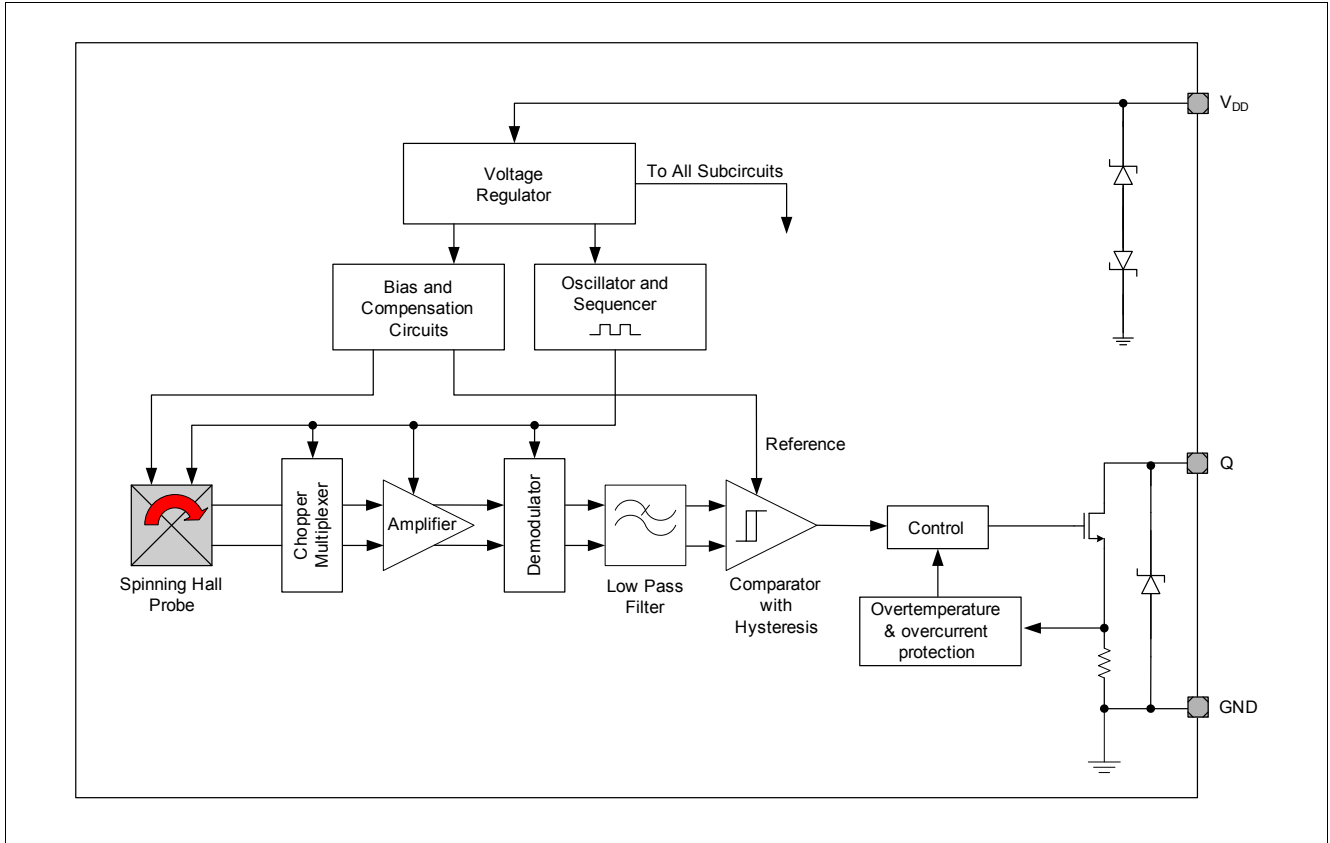
Figure 2-2 Functional Block Diagram TLE4961-3K
