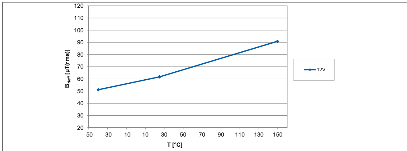
Figure 6-14 Effective Noise of the TLE4961-3K Thresholds over Temperature
