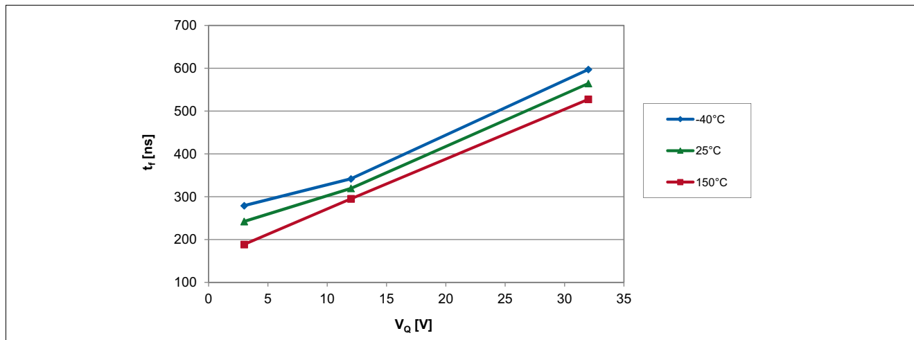
Figure 6-8 Output Fall Time of the TLE4961-3K over applied Pull-up Voltage
