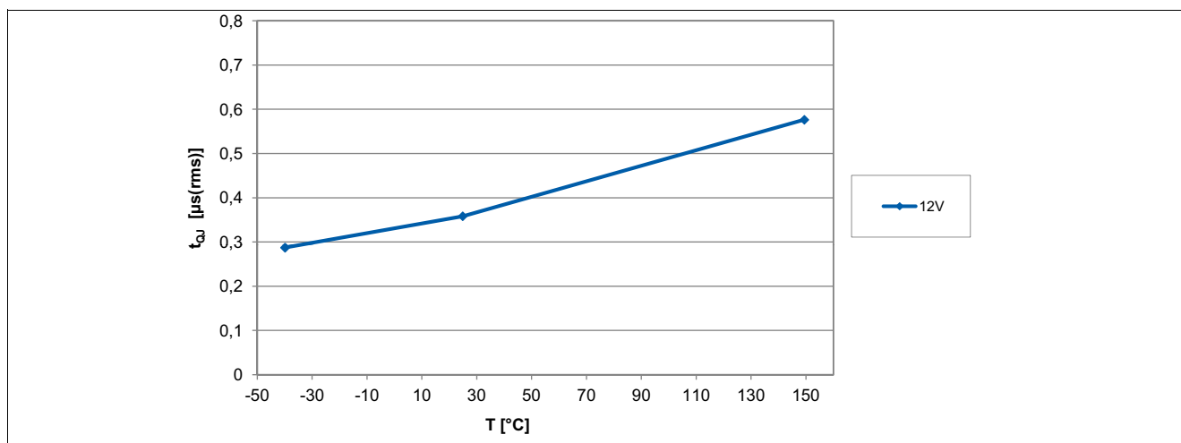
Figure 6-15 Output Signal Jitter of the TLE4961-3K over Temperature
