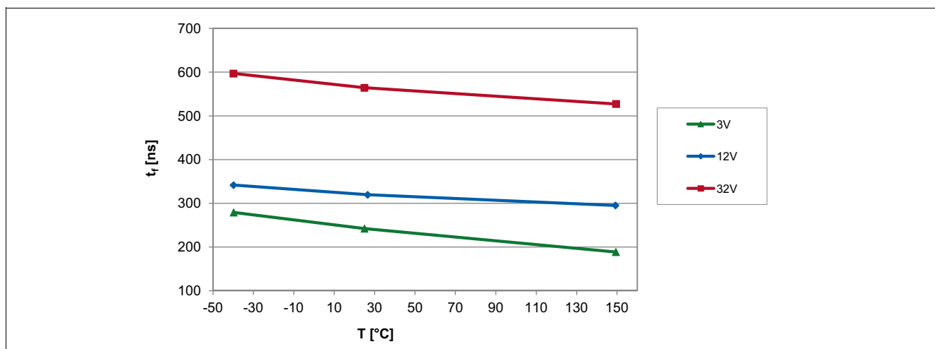
Figure 6-7 Output Fall Time of the TLE4961-3K over Temperature
