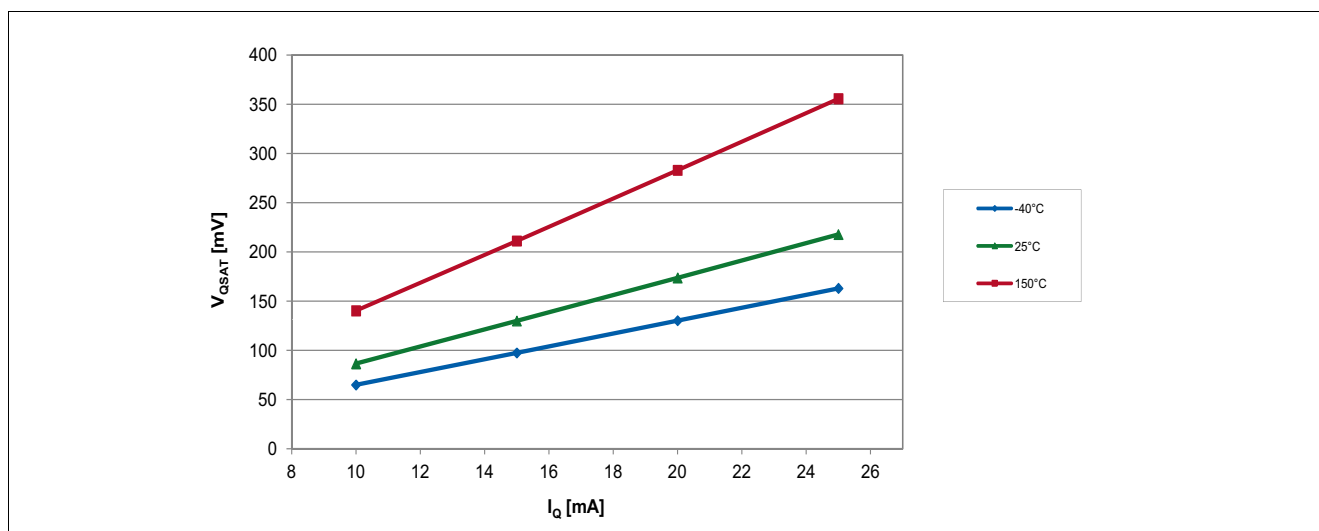
Figure 6-13 Saturation Voltage of the TLE4961-3K over Output Current
