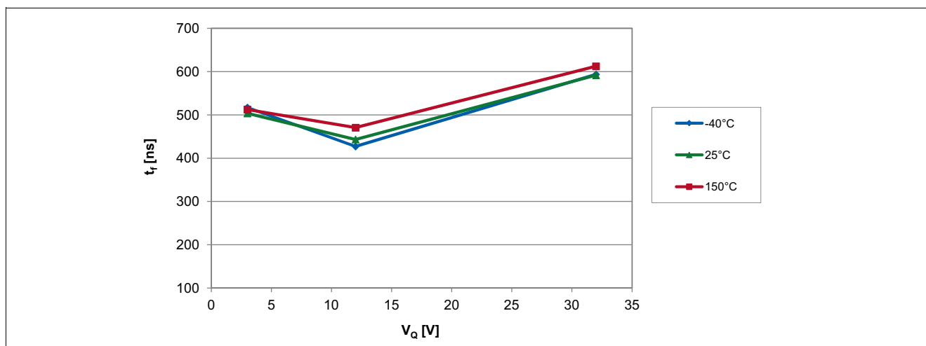
Figure 6-10 Output Rise Time of the TLE4961-3K over applied Pull-up Voltage
