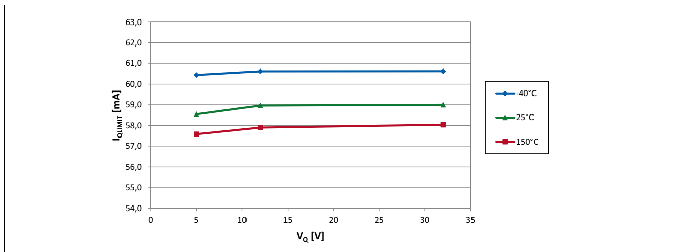
Figure 6-6 Output Current Limit of the TLE4961-3K over applied Pull-up Voltage
