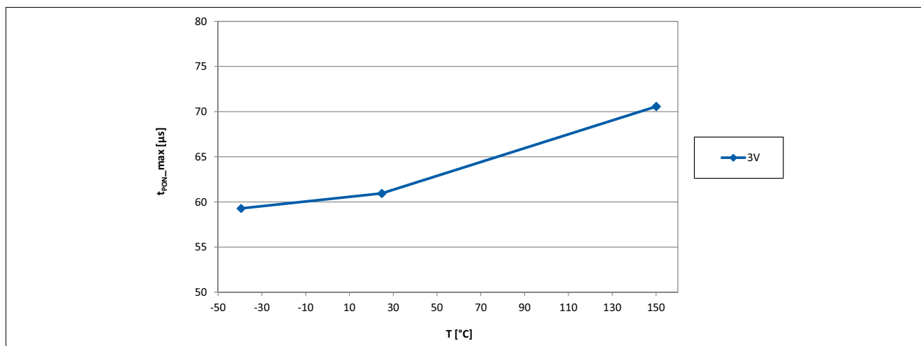
Figure 6-1 Power On Time t_{PON} of the TLE4961-3K over Temperature
