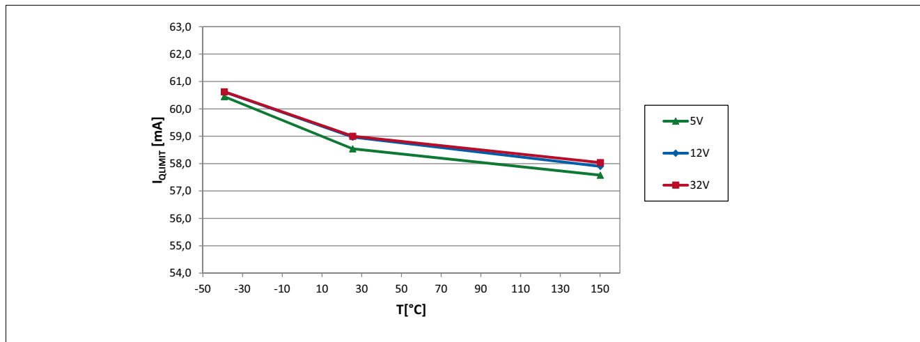
Figure 6-5 Output Current Limit of the TLE4961-3K over Temperature
