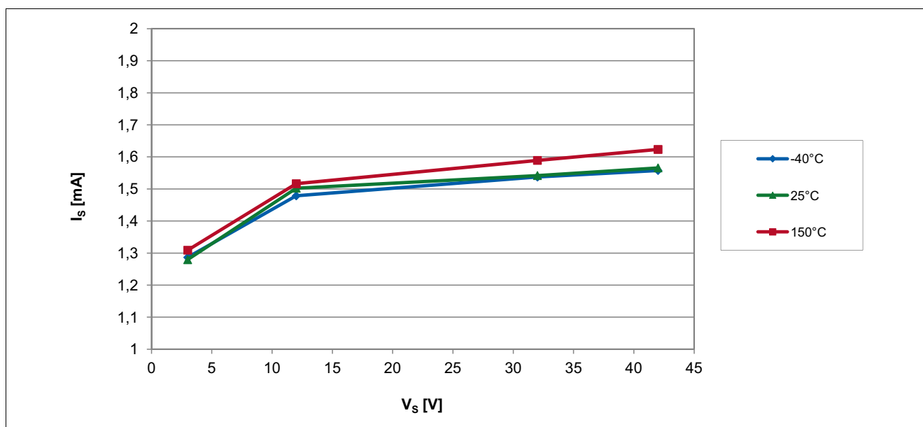
Figure 6-4 Supply Current of the TLE4961-3K over Supply Voltage
