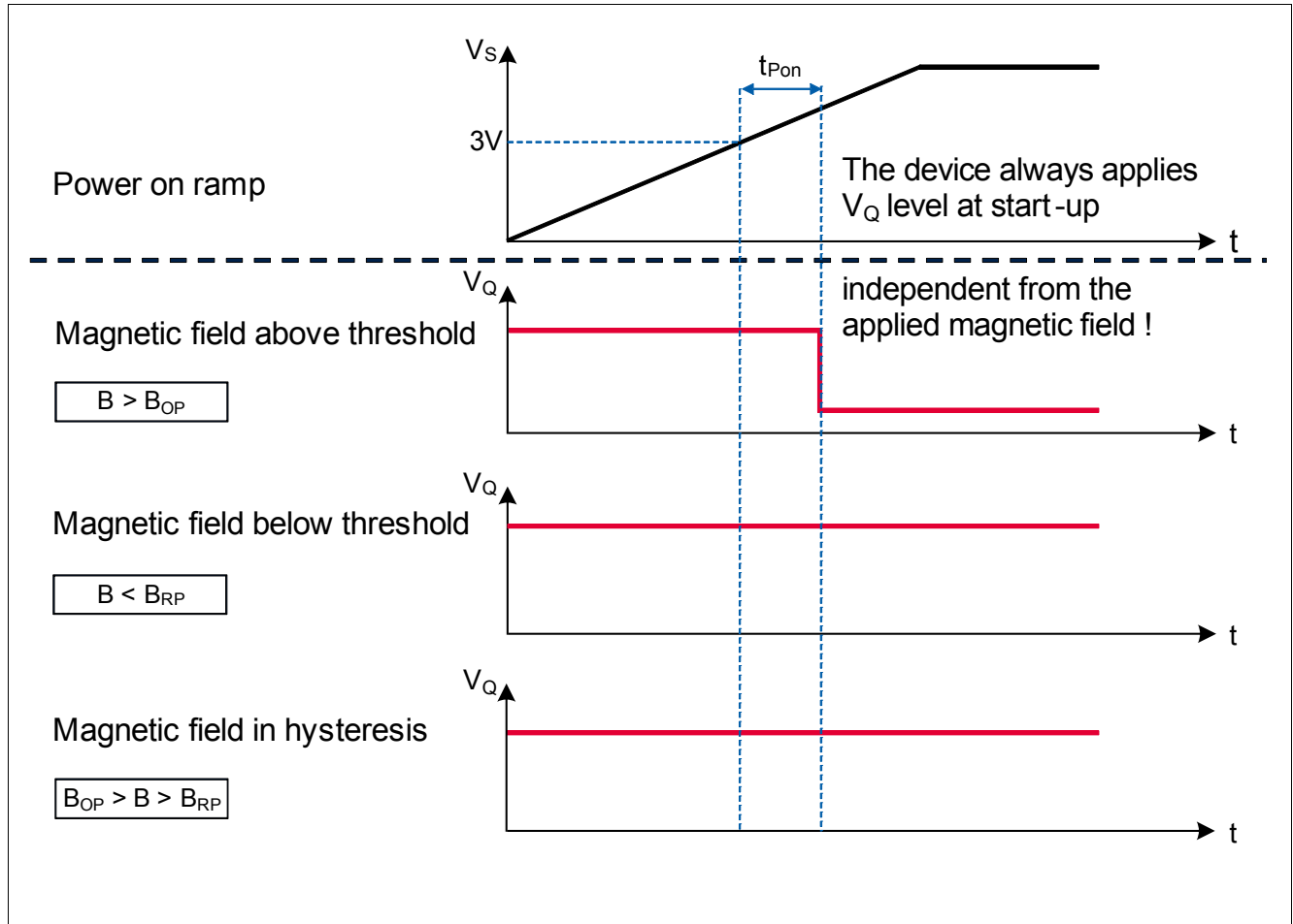
Figure 2-5 Illustration of the start-up behavior of the TLE4961-3K
