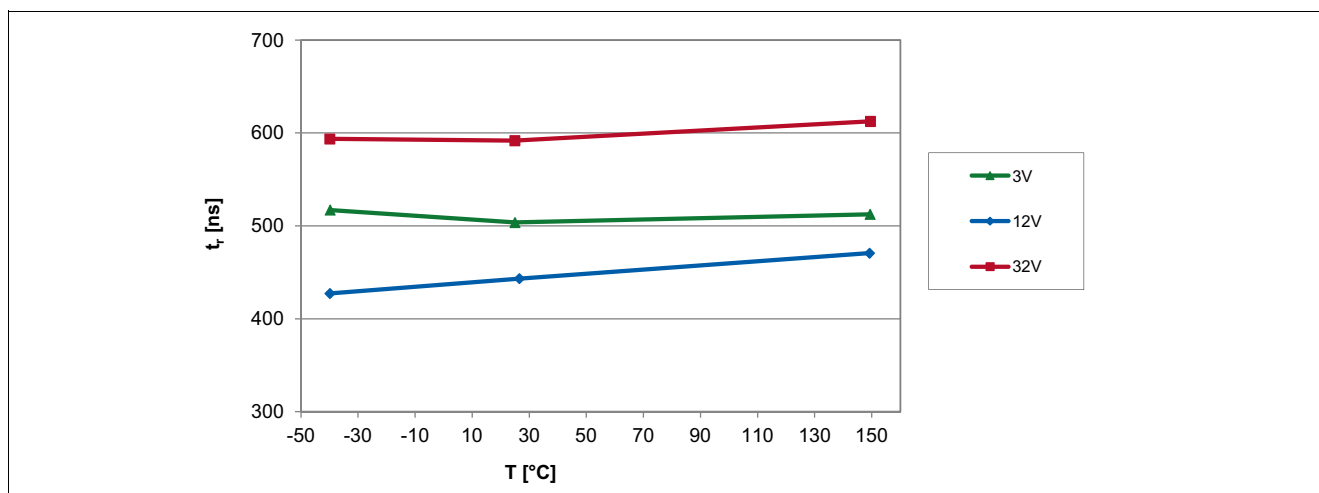
Figure 6-9 Output Rise Time of the TLE4961-3K over Temperature
