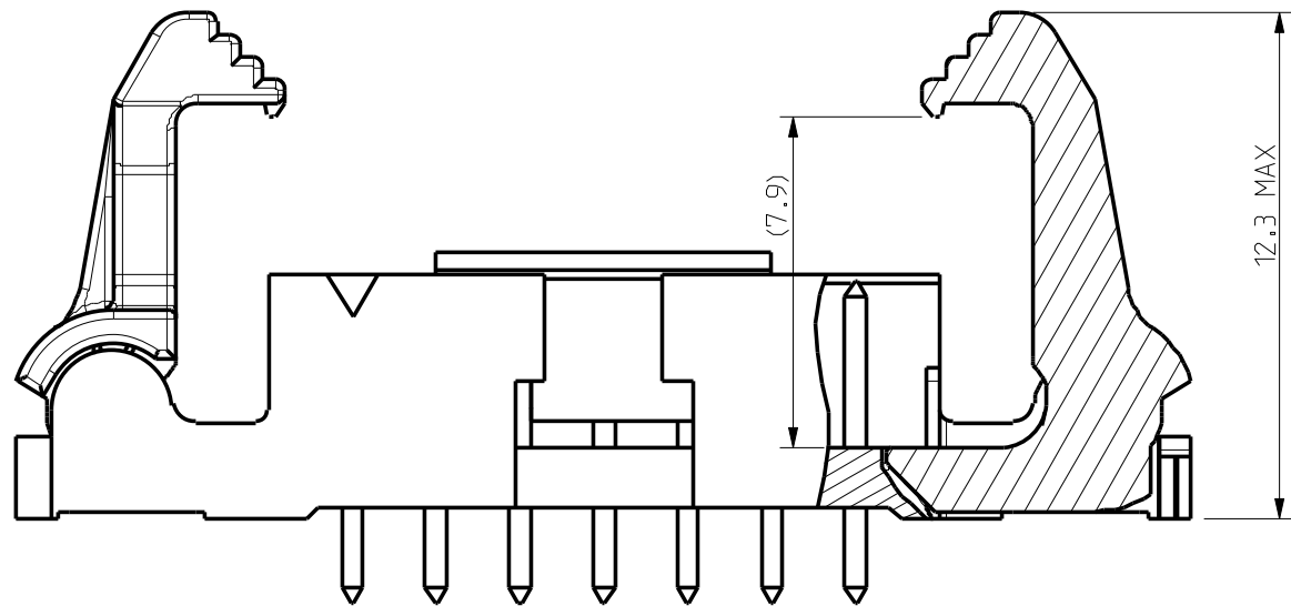
SECTION C-C
