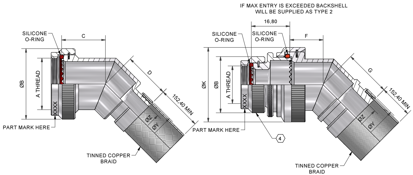
45° BACKSHELL - TYPE 1
