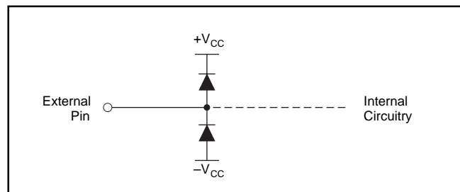
FIGURE 9. Internal ESD Protection.
