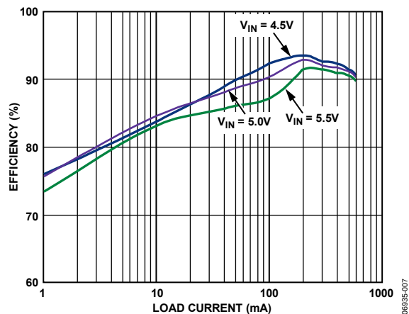
Figure 5. Efficiency vs. Load Current—ADP2102-4-EVALZ (3.3 V Output)
