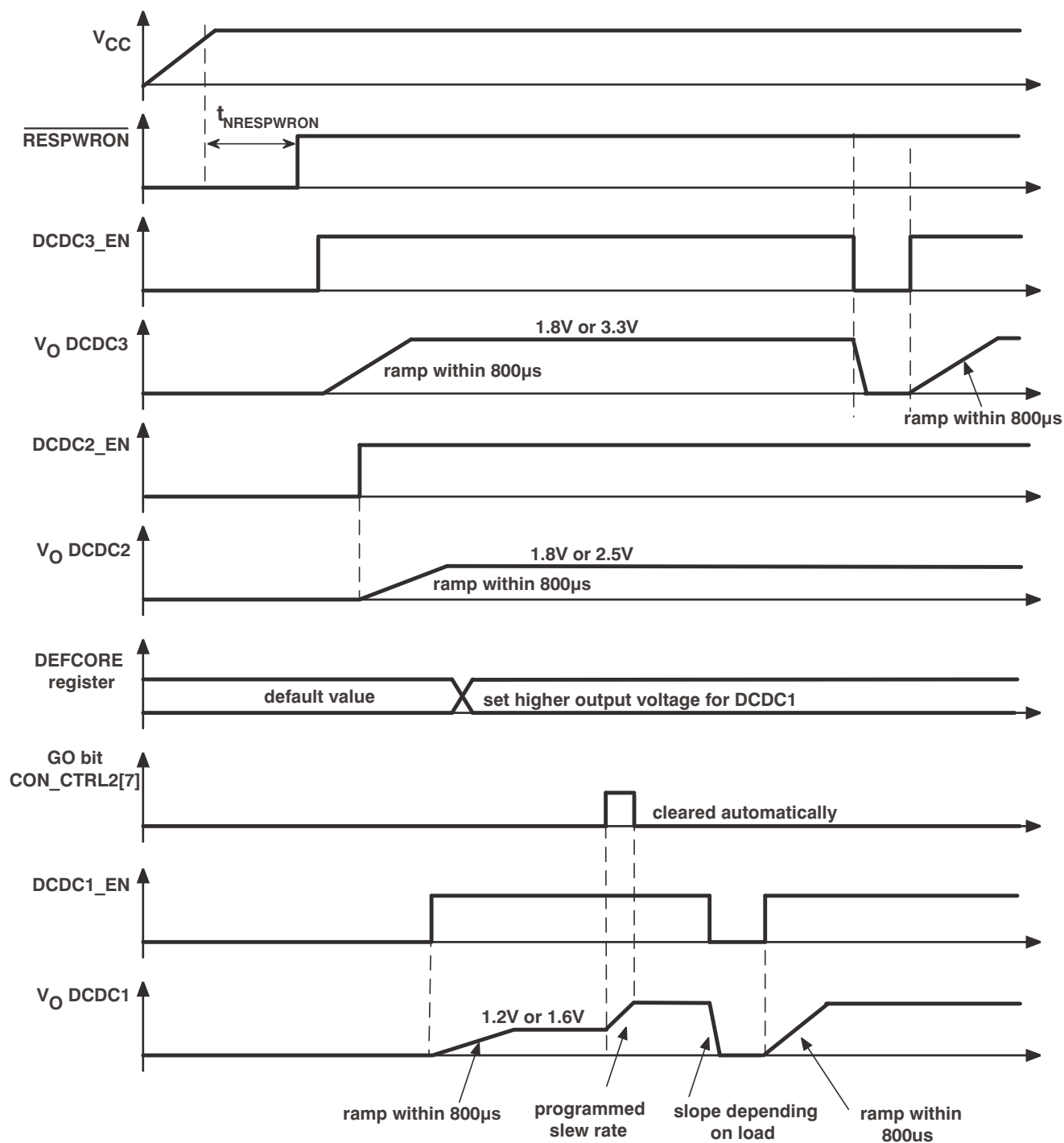
Figure 28. DVS Timing
