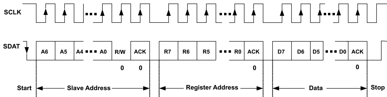
Figure 31. Serial i/f WRITE to TPS65023 Device
