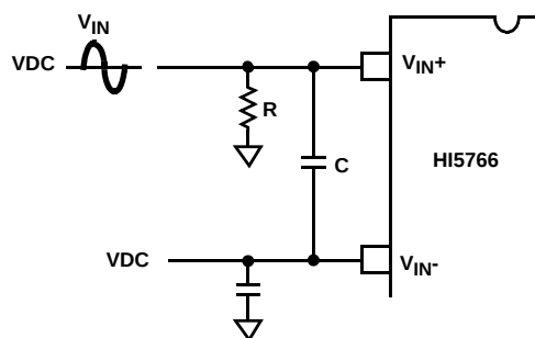
FIGURE 28. DC COUPLED SINGLE ENDED INPUT
