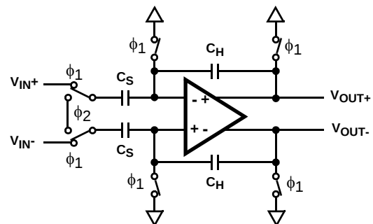
FIGURE 24. ANALOG INPUT SAMPLE-AND-HOLD
