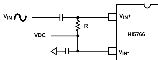
FIGURE 27. AC COUPLED SINGLE ENDED INPUT
