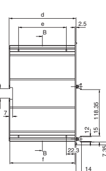
Section A – A Board depth 160 mm
