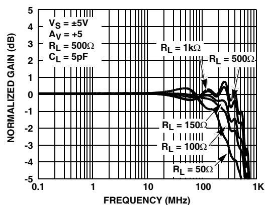
FIGURE 8. GAIN vs FREQUENCY FOR VARIOUS R_{LOAD}
