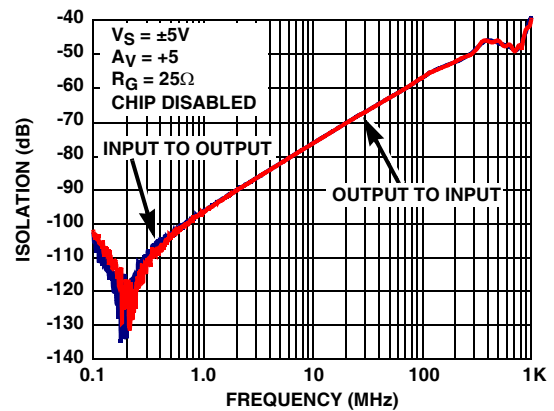
FIGURE 22. INPUT AND OUTPUT ISOLATION (EL5134, EL5234)
