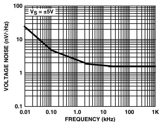
FIGURE 27. EQUIVALENT INPUT VOLTAGE NOISE vs FREQUENCY
