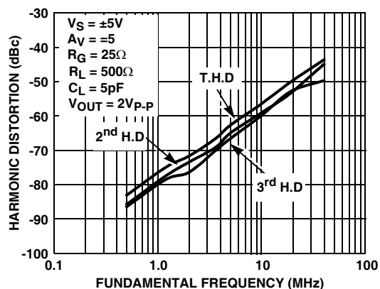
FIGURE 23. HARMONIC DISTORTION vs FREQUENCY
