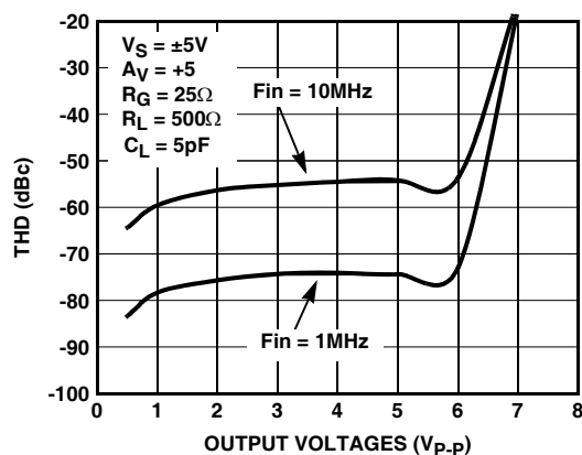
FIGURE 24. TOTAL HARMONIC DISTORTION vs OUTPUT VOLTAGES
