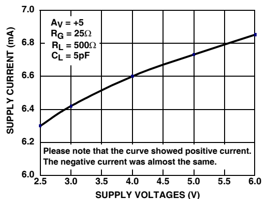
FIGURE 31. SUPPLY CURRENT vs SUPPLY VOLTAGE
