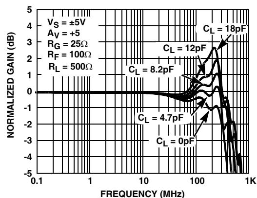
FIGURE 10. GAIN vs FREQUENCY FOR VARIOUS C_{LOAD} ( A_V = +5 )
