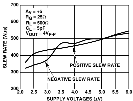
FIGURE 32. SLEW RATE vs SUPPLY VOLTAGES
