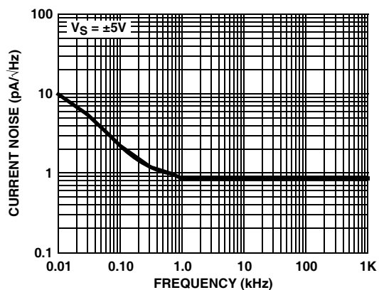
FIGURE 28. EQUIVALENT INPUT CURRENT NOISE vs FREQUENCY
