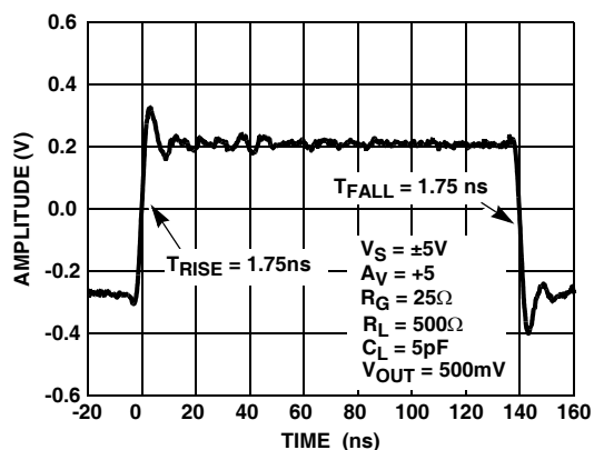
FIGURE 29. SMALL SIGNAL STEP RESPONSE_RISE AND FALL TIME
