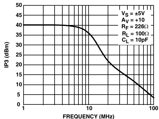
FIGURE 34. THIRD ORDER IMD INTERCEPT vs FREQUENCY
