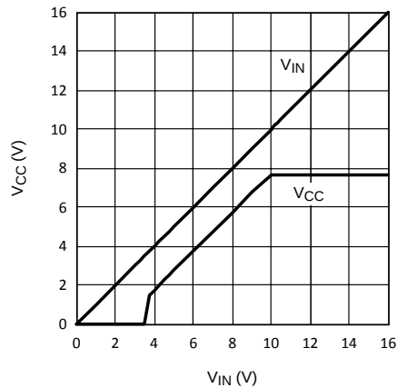
Figure 1. V_{CC} Regulator Start-Up Characteristics, V_{CC} vs V_{IN}
