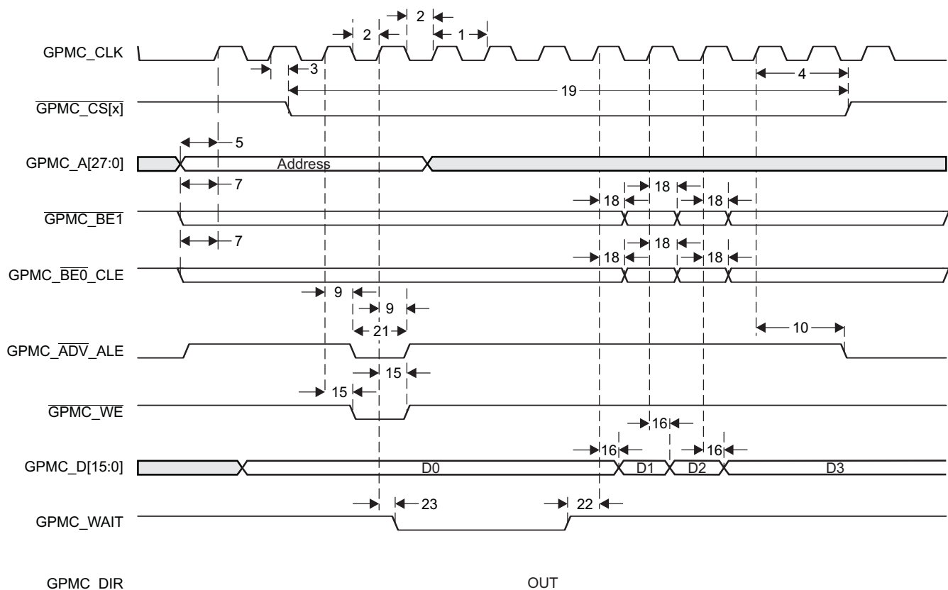
Figure 9-52. GPMC Non-Multiplexed NOR Flash - Synchronous Burst Write (GPMCFCLKDIVIDER = 0)
