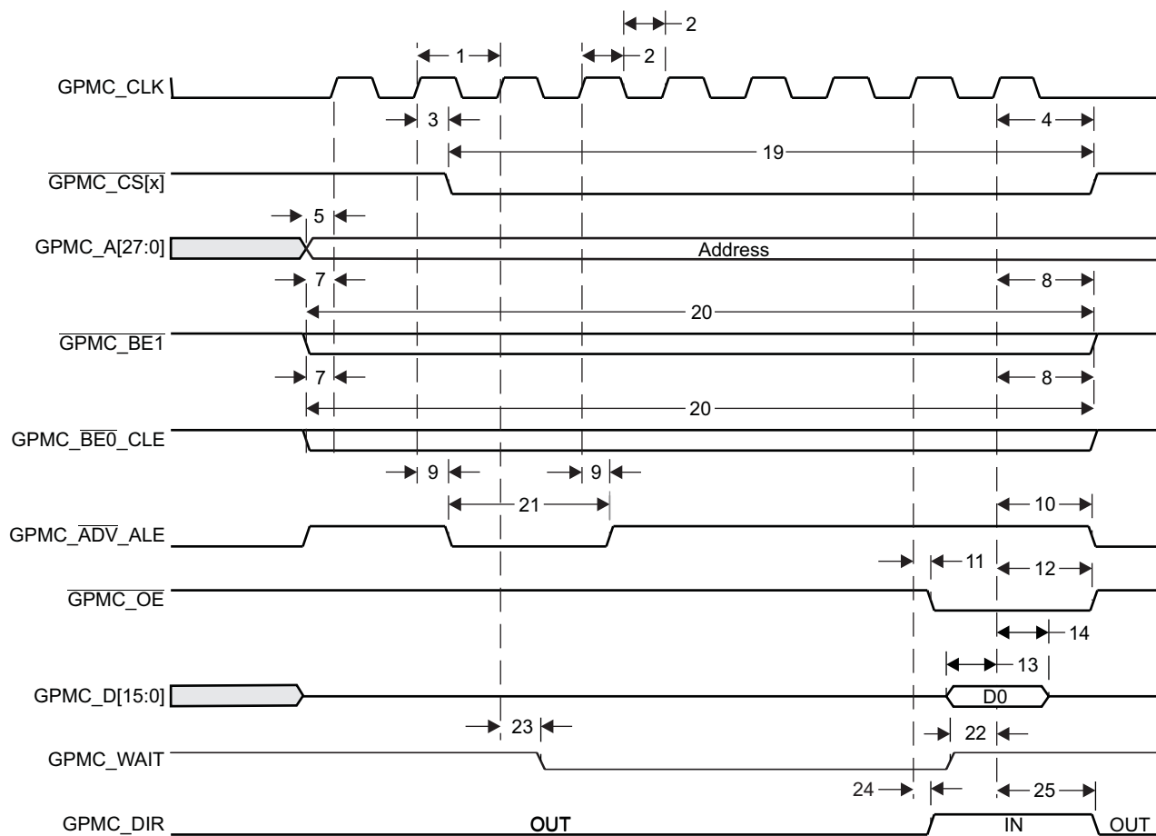
Figure 9-50. GPMC Non-Multiplexed NOR Flash - Synchronous Single Read (GPMCFCLKDIVIDER = 0)
