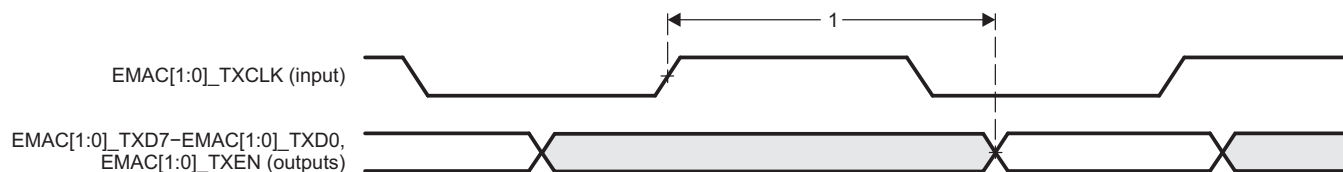
Figure 9-46. EMAC Transmit Timing
