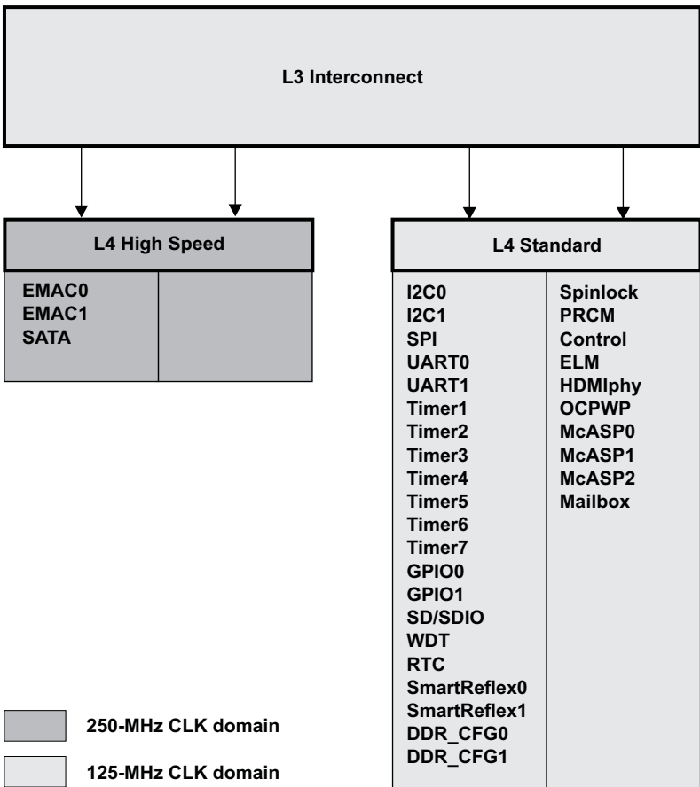
Figure 6-2. L4 Architecture
