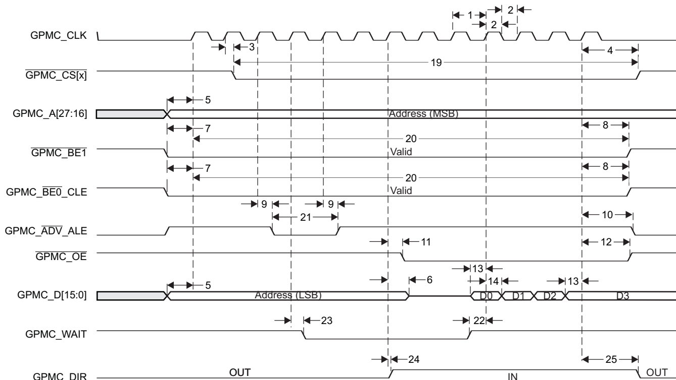
Figure 9-54. GPMC Multiplexed NOR Flash - 4x16-bit Synchronous Burst Read (GPMCCLKDIVIDER = 0)
