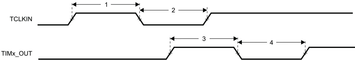
Figure 9-88. Timer Timing
