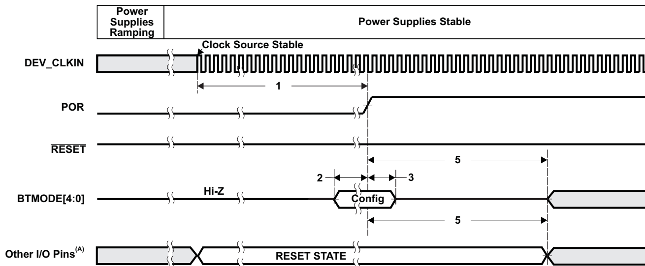
Figure 8-2. Power-Up Timing
