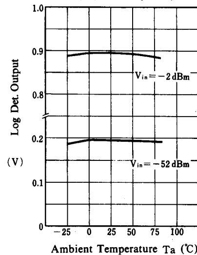
Log Detector Output
