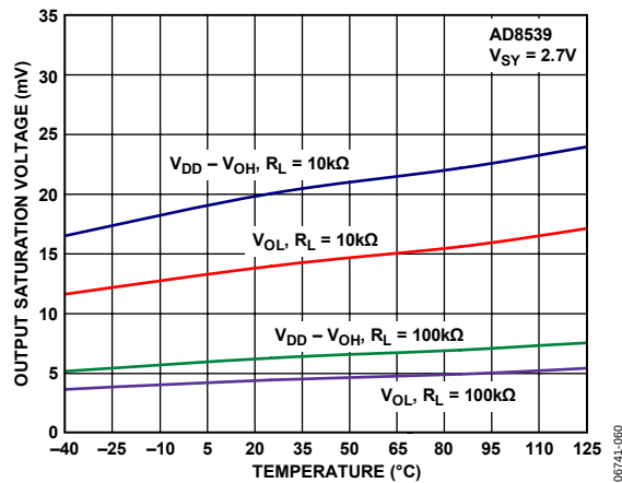
Figure 59. AD8539 Output Saturation Voltage vs. Temperature
