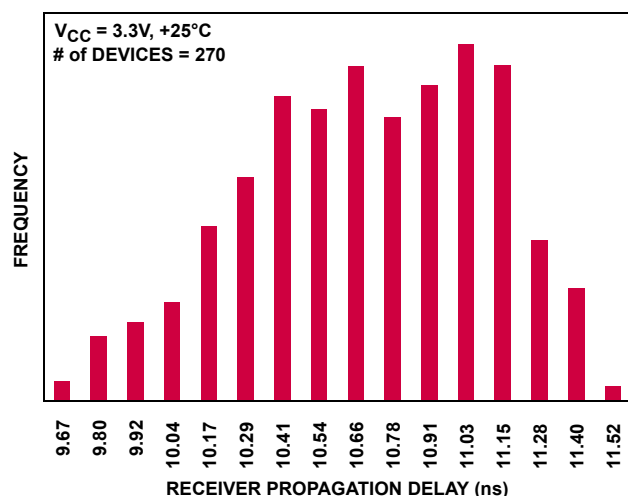
FIGURE 1. ISL32177E PART-TO-PART PROP DELAY VARIABILITY
