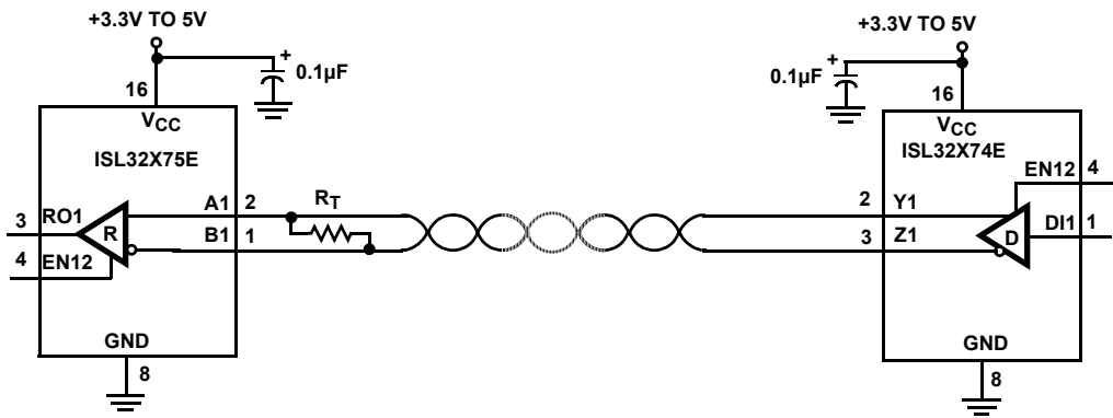
FIGURE 4. NETWORK USING PAIRED ENABLES
