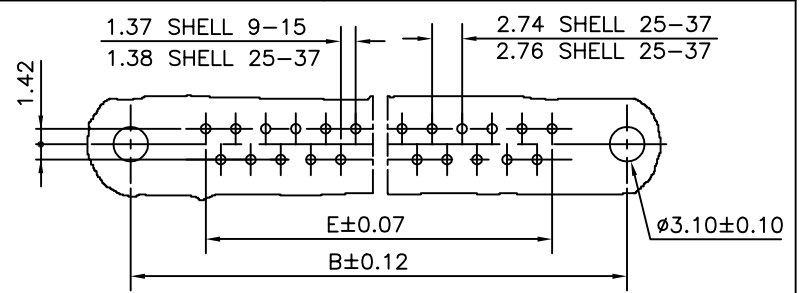
PCB DRILLING DETAILS
