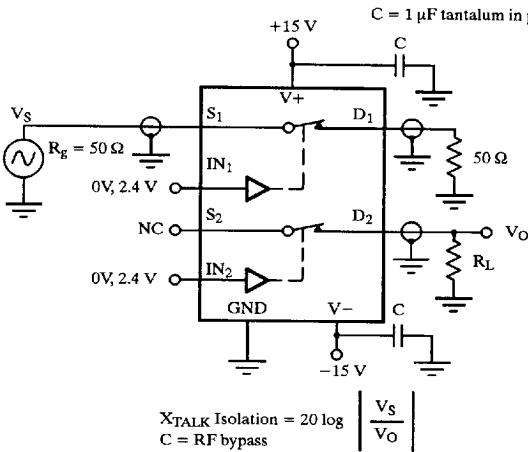
Figure 4. Crosstalk
