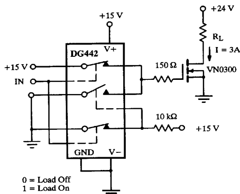
Figure 7. Power MOSFET Driver
