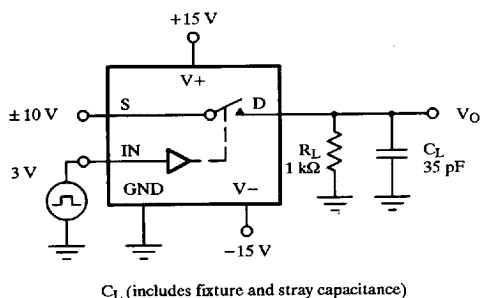
Figure 2. Switching Time
