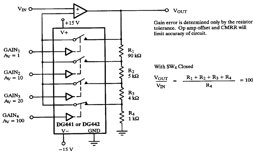
Figure 9. Precision-Weighted Resistor Programmable-Gain Amplifier
