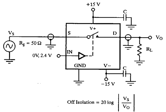
Figure 5. Off Isolation
