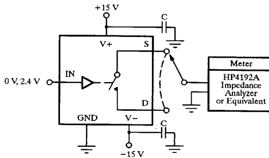
Figure 6. Source/Drain Capacitances
