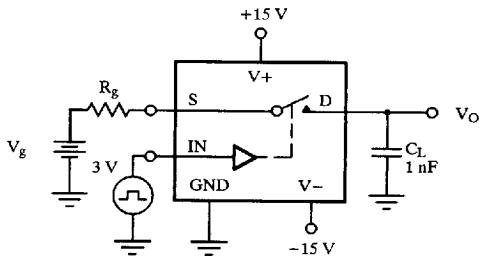
Figure 3. Charge Injection
