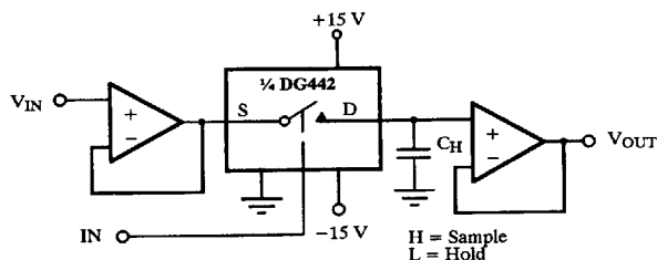
Figure 8. Open Loop Sample-and-Hold
