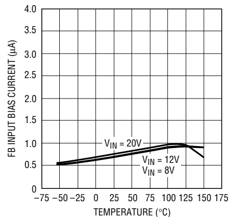
FB Input Bias Current vs Temperature
