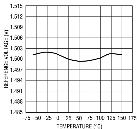
LT1575-1.5 V_{OUT} vs Temperature
