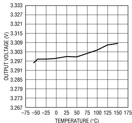
LT1575-3.3 V_{OUT} vs Temperature
