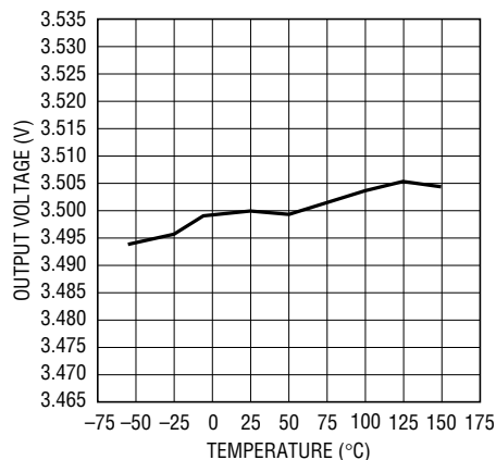
LT1575-3.5 V_{OUT} vs Temperature
