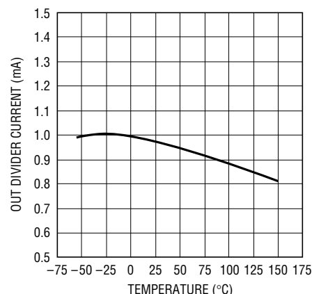
OUT Divider Current vs Temperature
