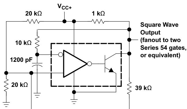
Figure 16. 100-kHz Free-Running Multivibrator
