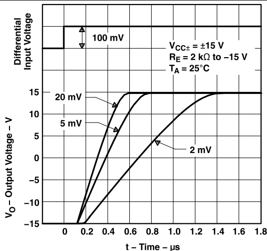
Figure 14. Output Response for Various Input Overdrives
