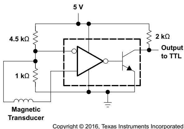
Figure 19. TTL Interface With High-Level Logic
