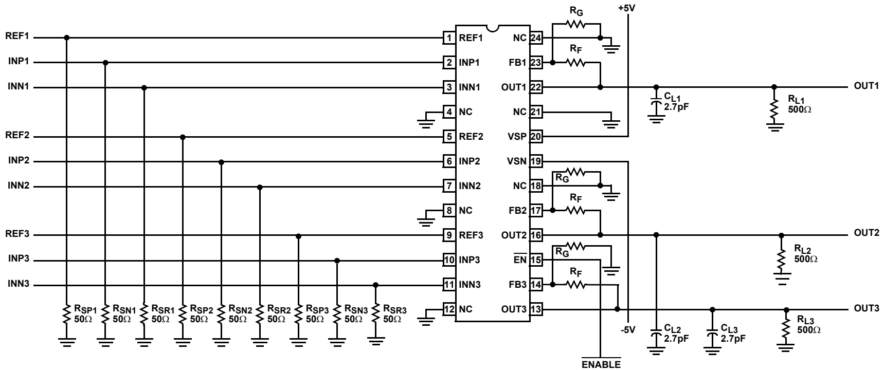
FIGURE 2. EL5375
