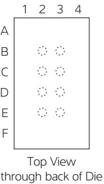
Figure 2-3. 8-dBGA
