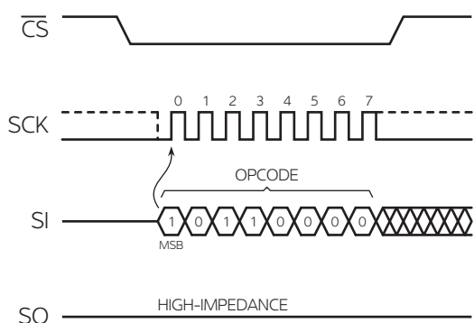
Figure 8-7. Program/Erase Suspend
