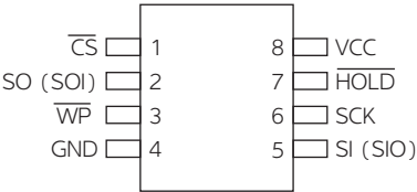
Figure 2-1. 8-SOIC (Top View)
