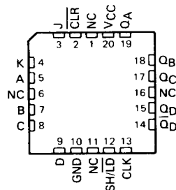
SN54HC195 . . . FK PACKAGE (TOP VIEW)
