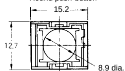
Round push-button
