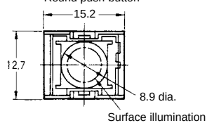
Round push-button
