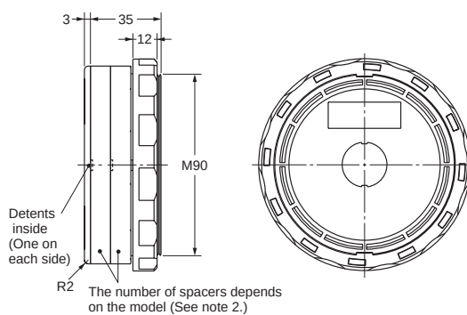
Mounting a 1-pole Switch Unit (See note 5.)
