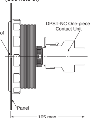
Mounting a 2-pole Switch Unit (See note 5.)
