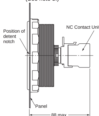
Mounting a 1-pole Switch Unit (See note 5.)
