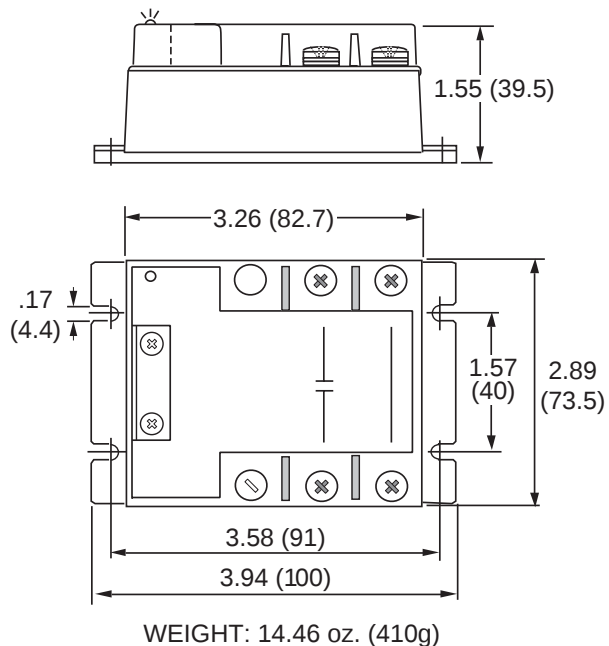
Figure 1 – EPC relays; dimensions in inches (mm)
