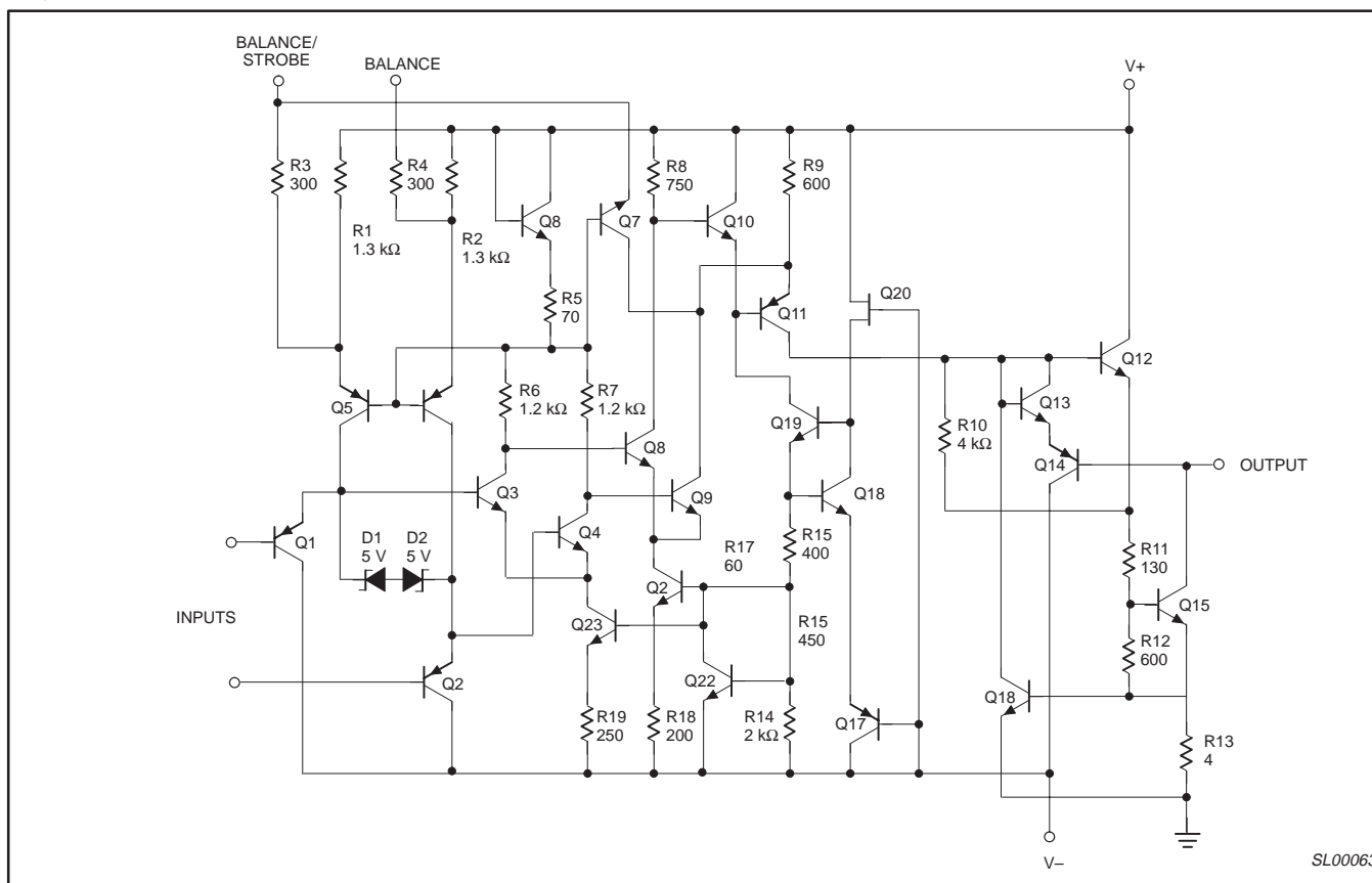
Figure 2. Equivalent Schematic
