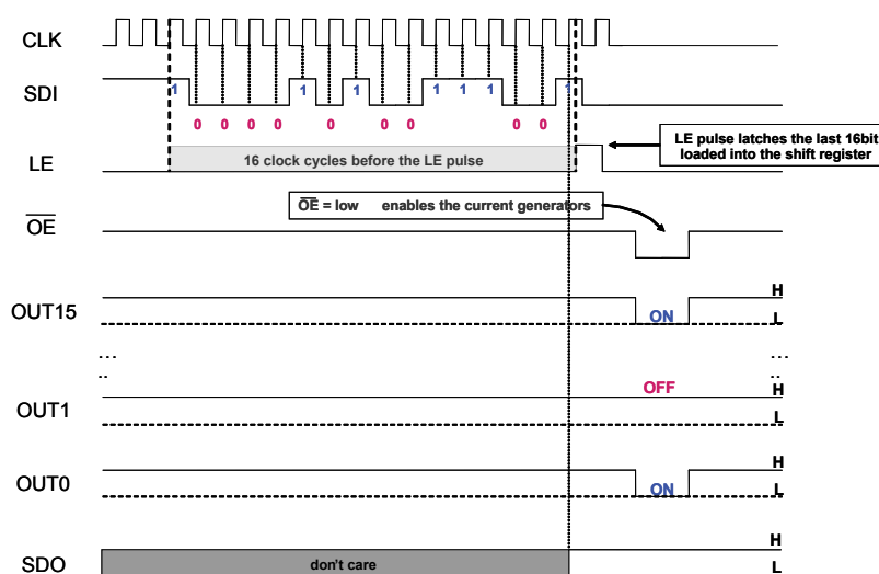
Figure 10. Timing diagram
