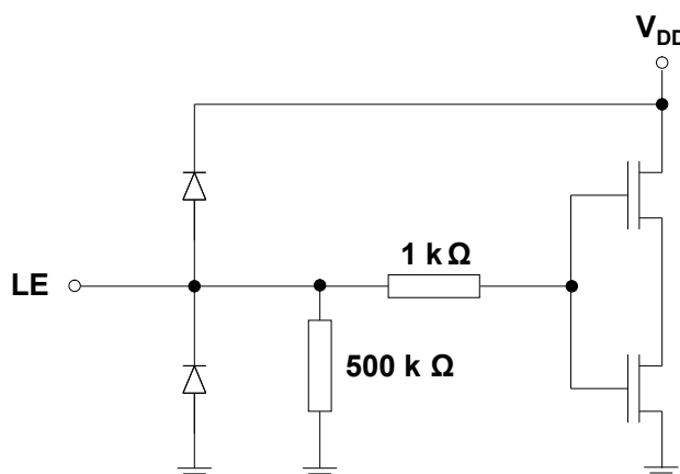
Figure 5. LE terminal
