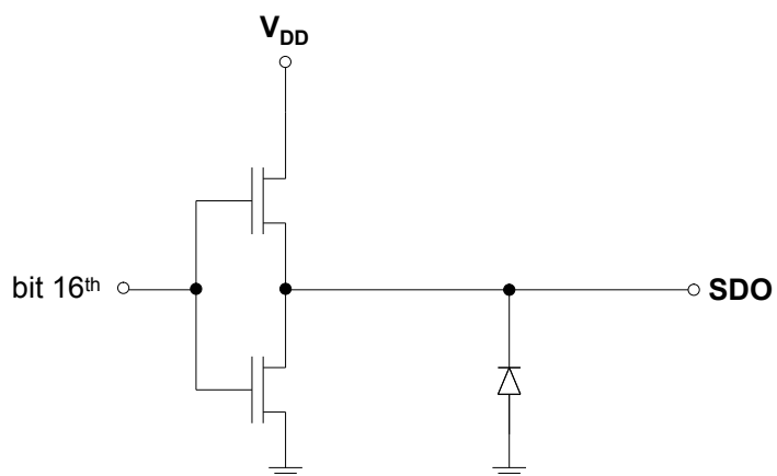
Figure 7. SDO terminal
