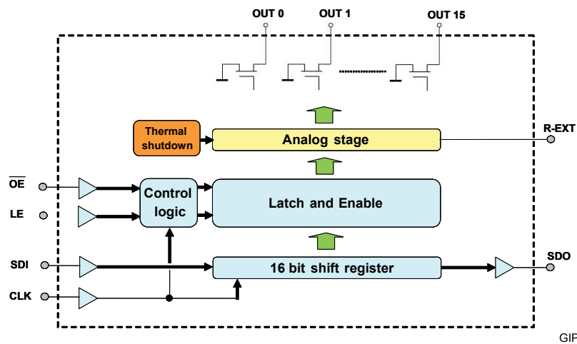
Figure 2. STP16CPC26 simplified block diagram
