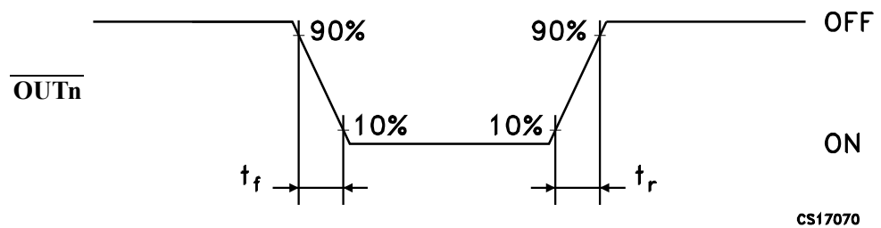
Figure 13. Outputs
