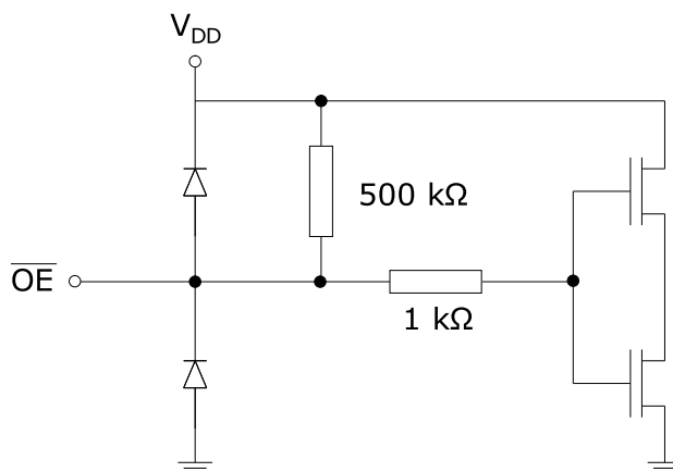
Figure 4. \overline{\text{OE}} terminal
