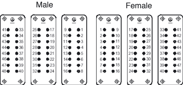
view from cable side
