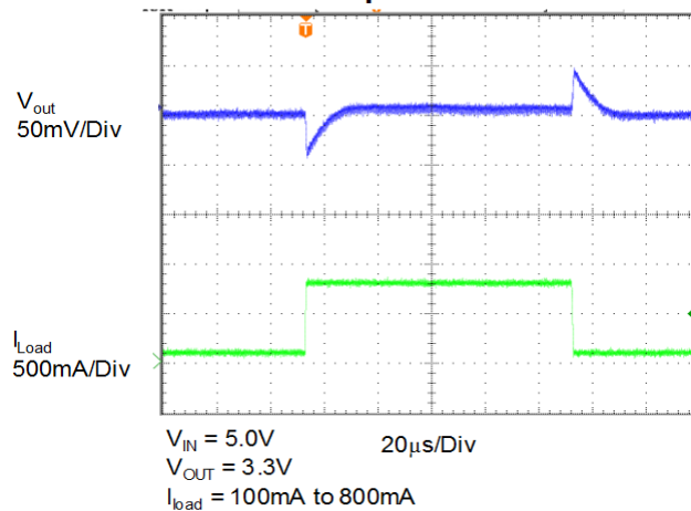
Transient Response
