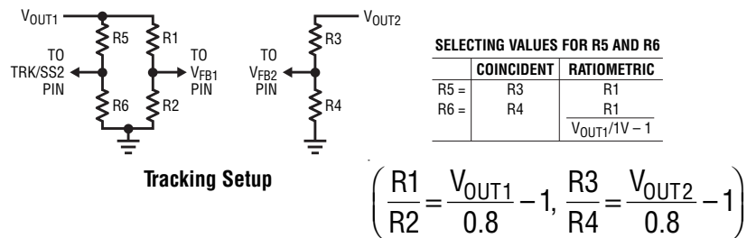
Figure 9. Setup for Coincident and Ratiometric Tracking
