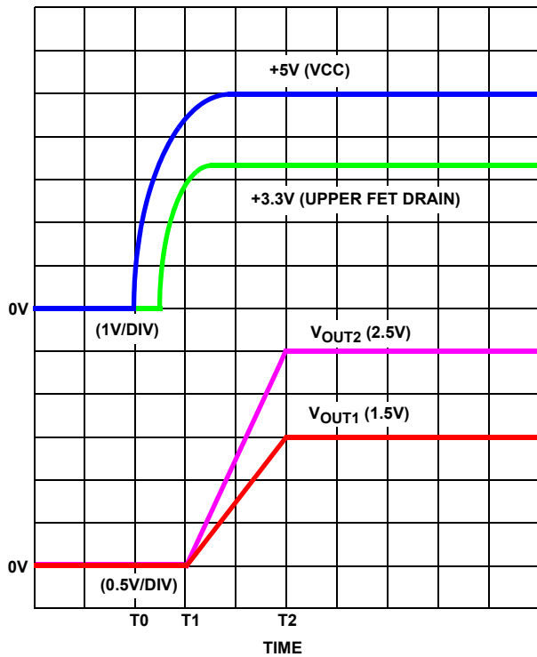
FIGURE 1. SOFT-START INTERVAL
