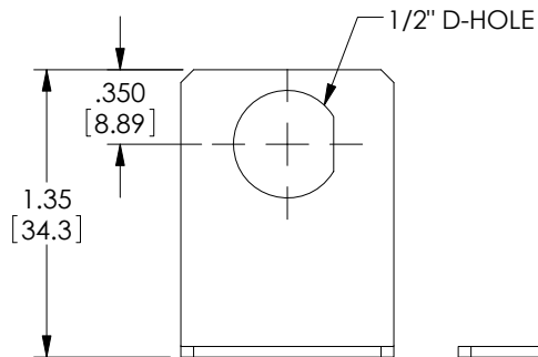
MOUNTING BRACKET
