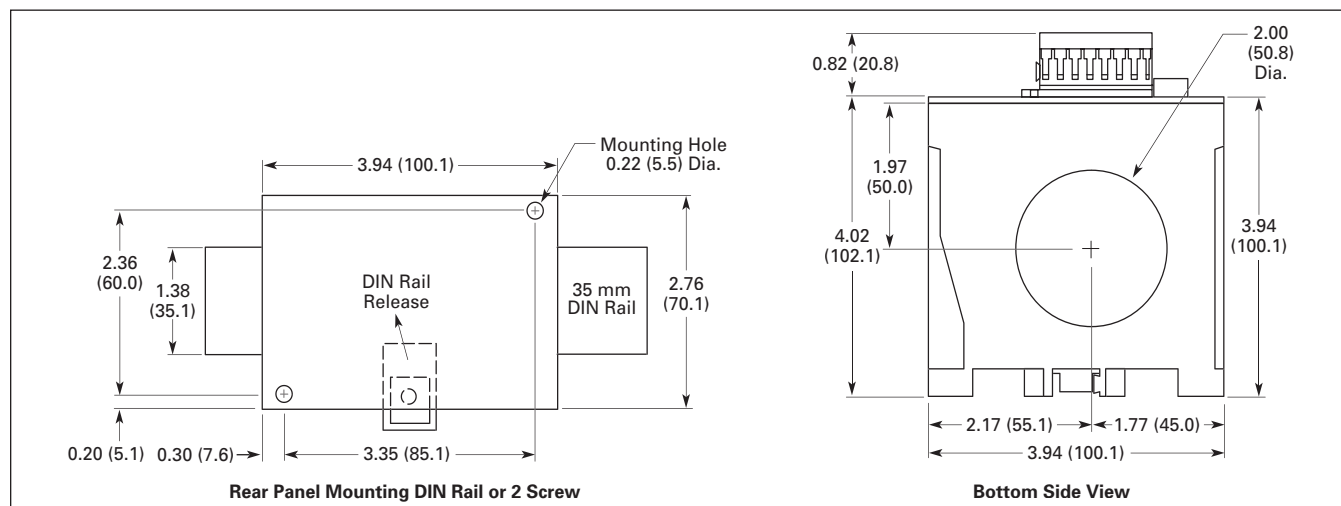
Figure 32.2-9. D64RPB100—Approximate Dimensions in Inches (mm)
