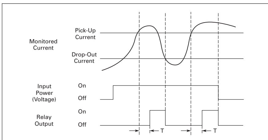
Figure 32.2-18. Overcurrent Monitoring
