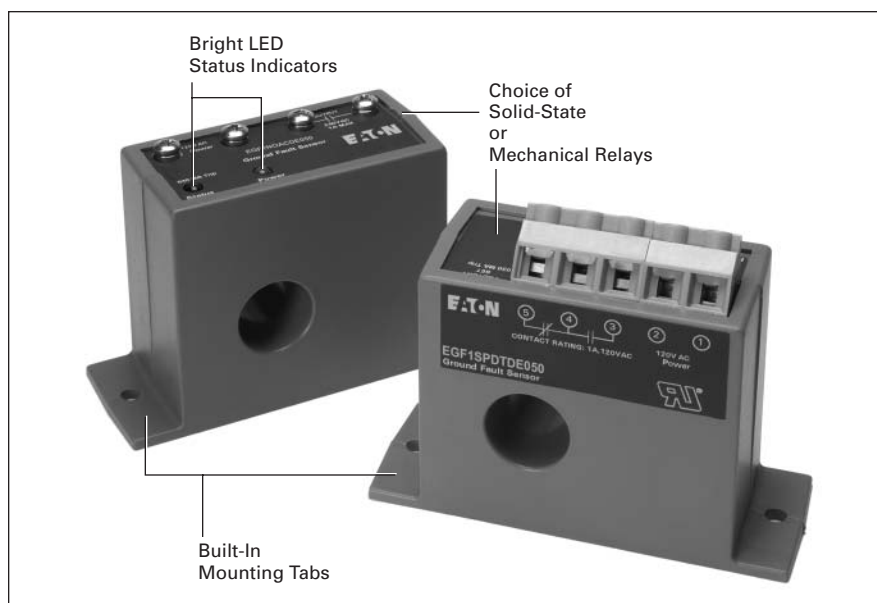
Figure 32.2-13. Ground Fault Sensors with Solid-State or Mechanical Relay Outputs
