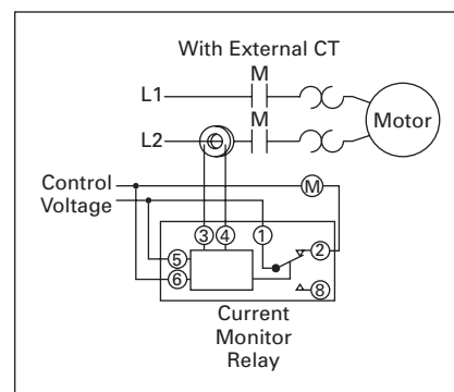
Figure 32.2-16. Typical Installation with External CT
