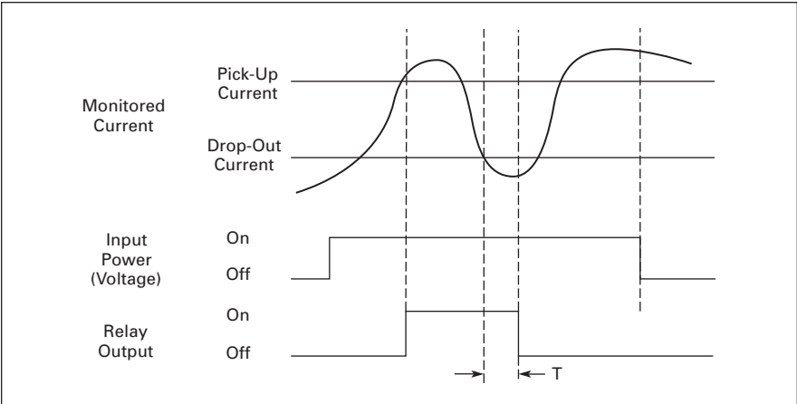
Figure 32.2-19. Undercurrent Monitoring
