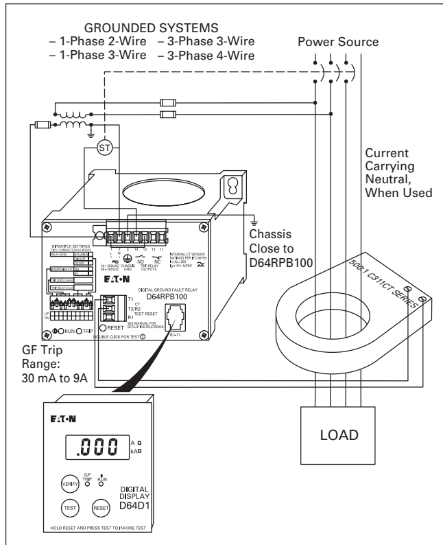
Figure 32.2-5. Typical Field Connection of D64RPB100 with External 500:1 Current Transformer (C311CT Series) Pulsed Trip-Auto Reset for Shunt Breaker
