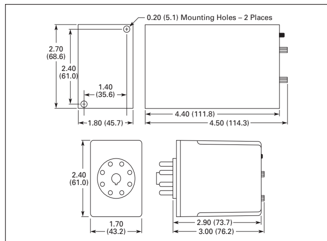
Figure 32.3-1. Surface-Mount and Plug-In—Approximate Dimensions in Inches (mm)
