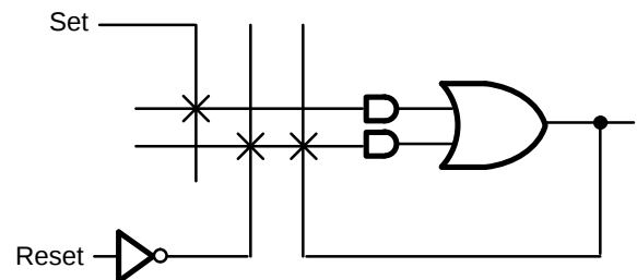
Figure 3. Combinatorial Latch
