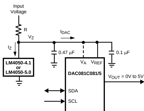
Figure 33. The LM4050 as a Power Supply
