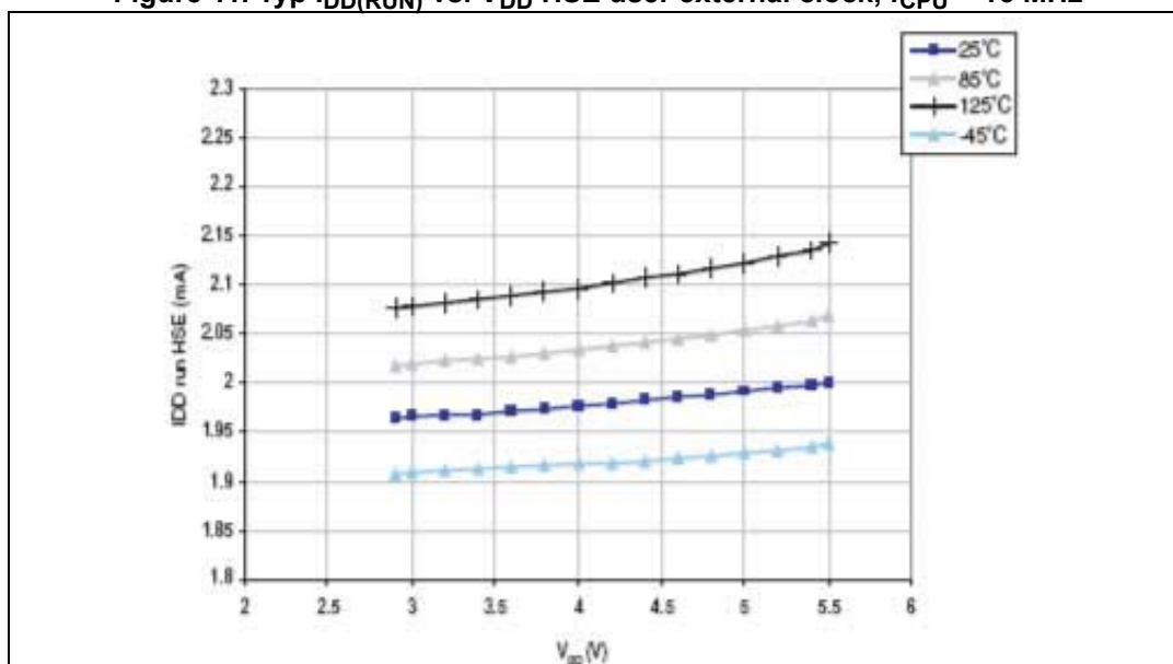
Figure 11. Typ I_{\text{DD(RUN)}} vs. V_{\text{DD}} HSE user external clock, f_{\text{CPU}} = 16 \text{ MHz}
