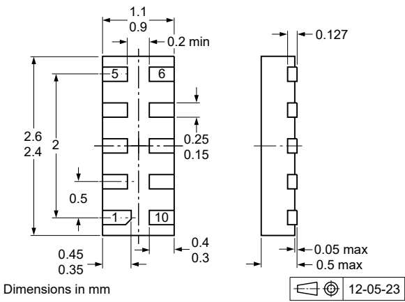
Fig. 15. Package outline DFN2510A-10 (SOT1176-1)
