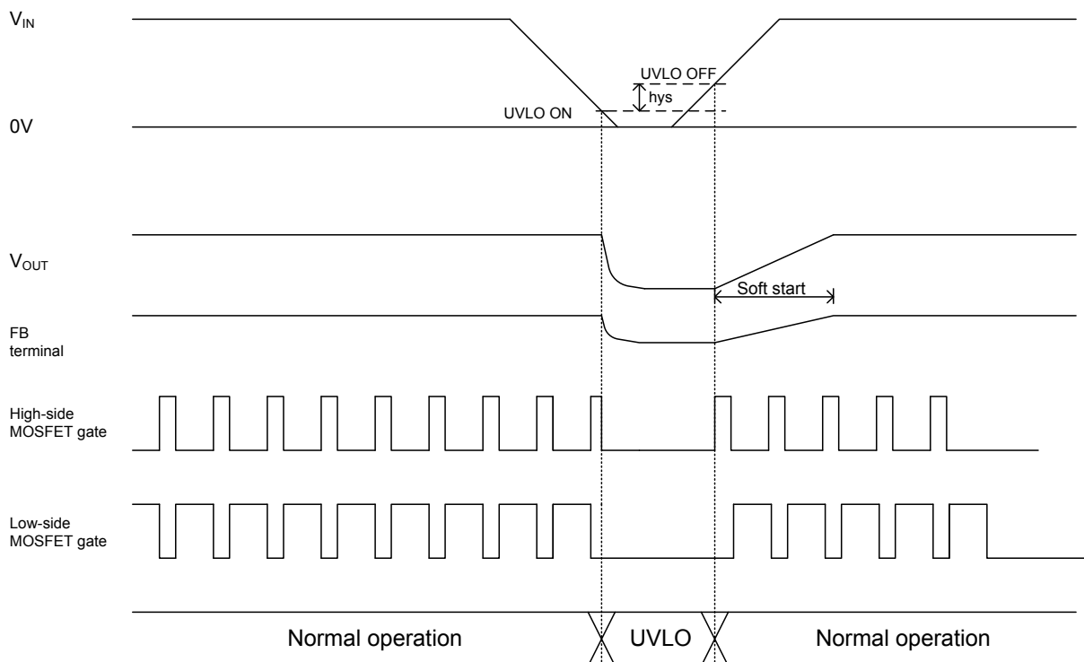
Figure 39. UVLO Timing Chart
