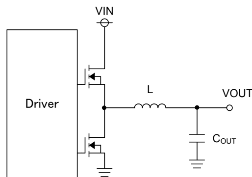
Figure 43. Output LC filter circuit
