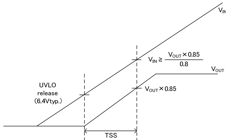
Figure 45. Input Voltage Start-up Time
