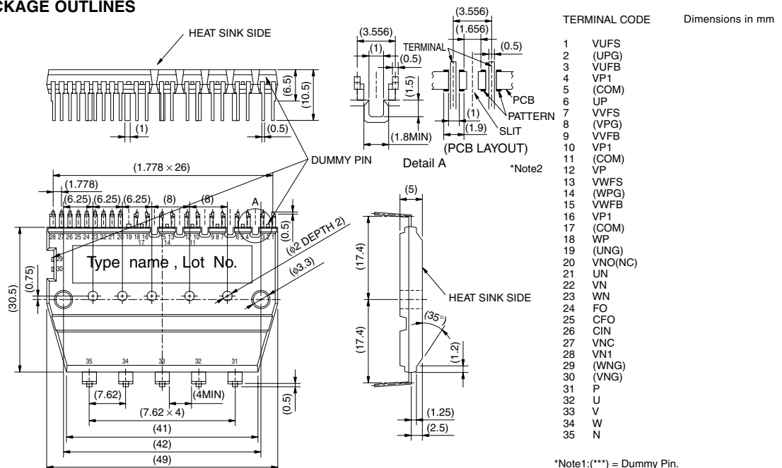
Fig. 1 PACKAGE OUTLINES
