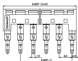
Dimensions - mm
