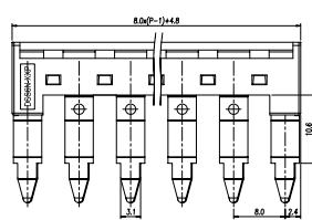
Dimensions - mm
