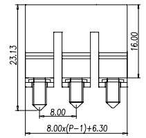
Dimensions - mm
