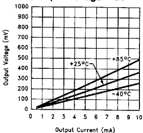
Output Sinking Current vs Output Voltage @ 5V
