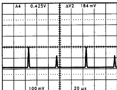
FIGURE 3. Measurement of the Shoot-Through Current
