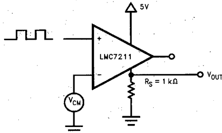
FIGURE 2. Circuit for Measurement of the Shoot-Through Current
