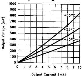
Output Sourcing Current vs Output Voltage @ 15V
