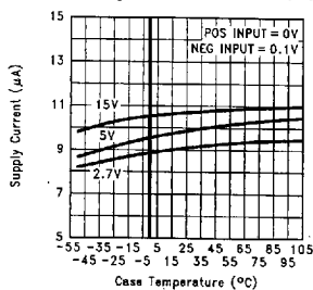
Supply Current vs Temperature while Sourcing
