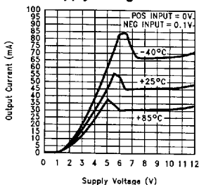
Output Sinking Current vs Supply Voltage
