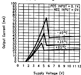
Output Sourcing Current vs Supply Voltage
