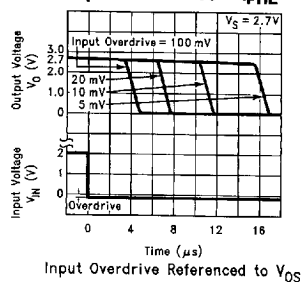
Response Time for Various Input Overdrives - t_{PHL}
